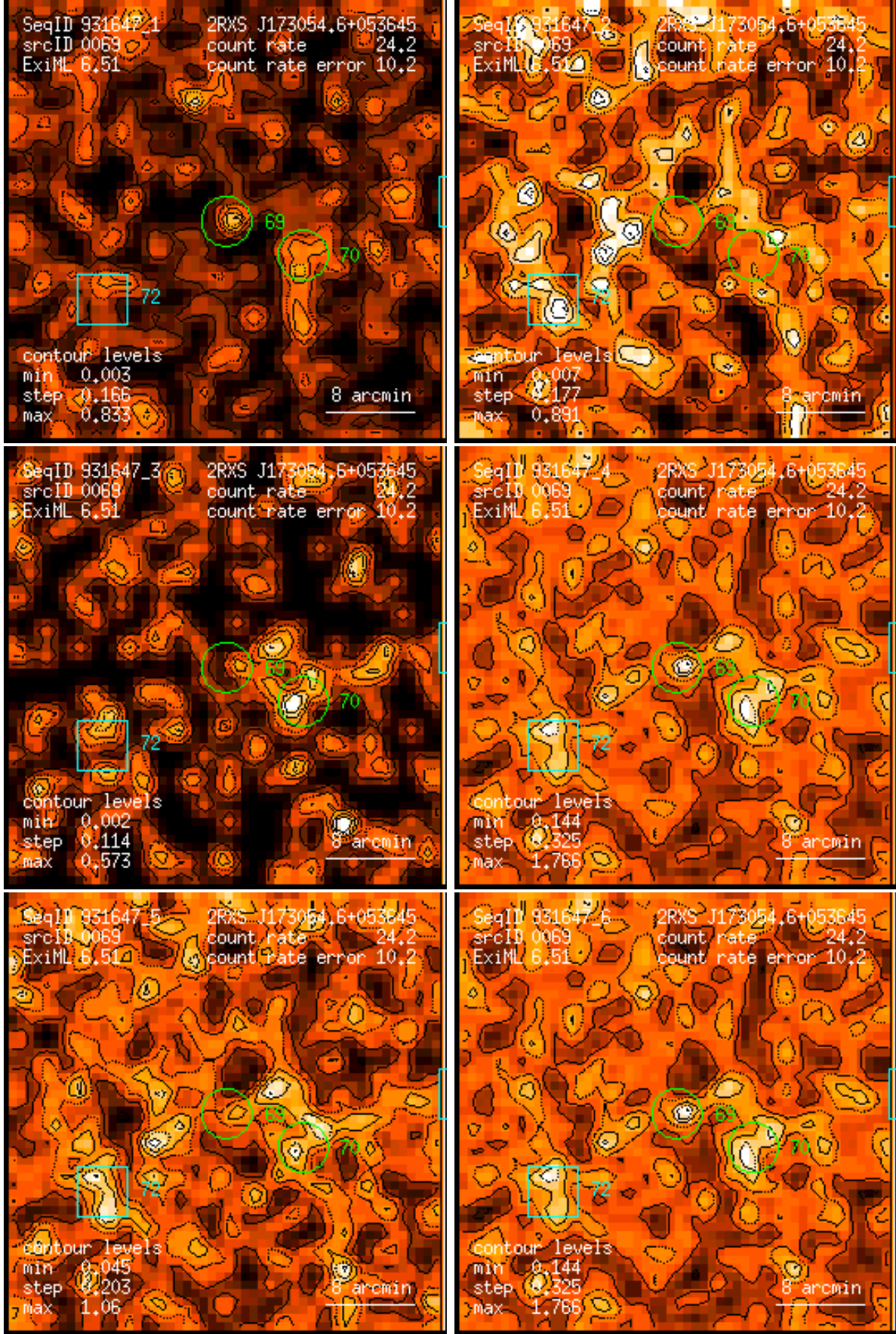
Figure 69: RASS 931647: detection 0069: band rate images, Gaussian filter: (1) PSPC channels 11 – 41, (2) 52 – 90, (3) 91 – 201, (4) 11 – 235, (5) 52 – 201, (6) 11 – 201. Broad band rates in counts/ks. Band rate contour levels in counts/ks/arcmin 2 .
