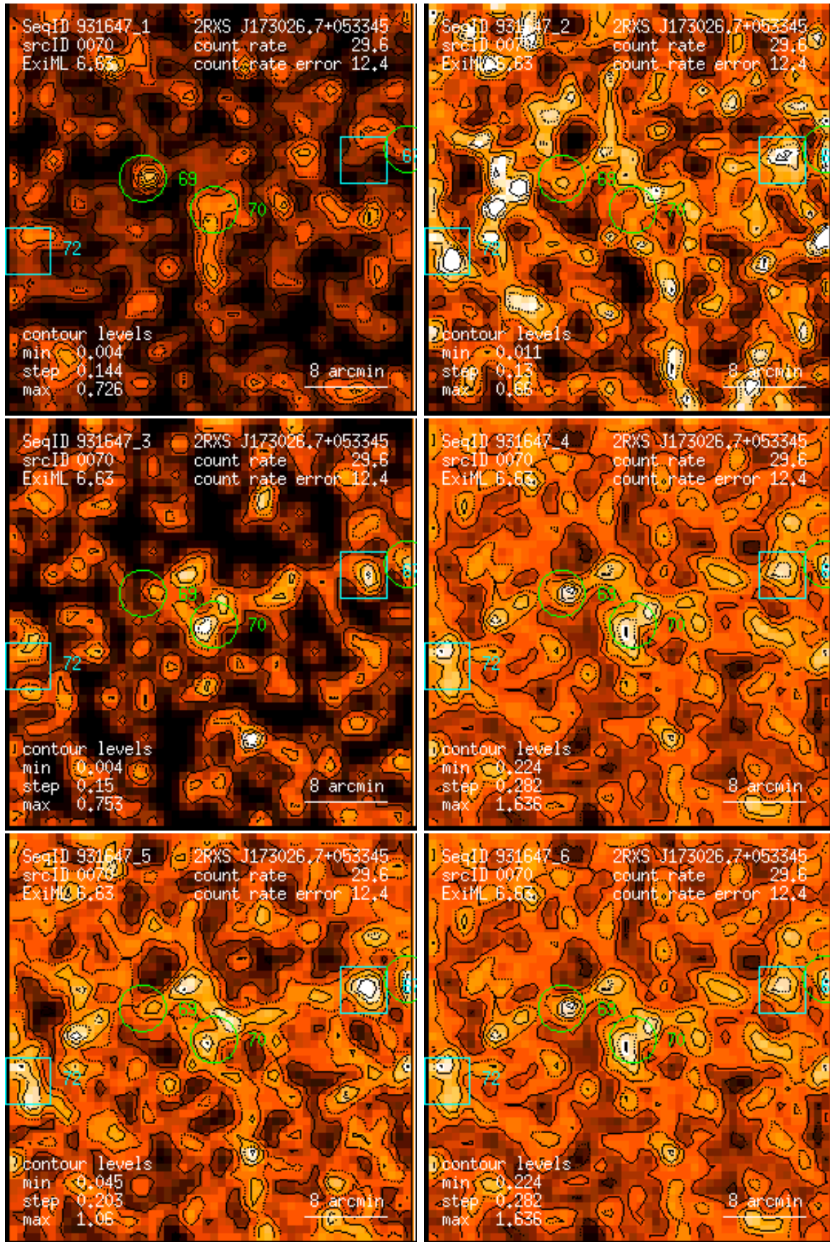
Figure 70: RASS 931647: detection 0070: band rate images, Gaussian filter: (1) PSPC channels 11 – 41, (2) 52 – 90, (3) 91 – 201, (4) 11 – 235, (5) 52 – 201, (6) 11 – 201. Broad band rates in counts/ks. Band rate contour levels in counts/ks/arcmin 2 .
