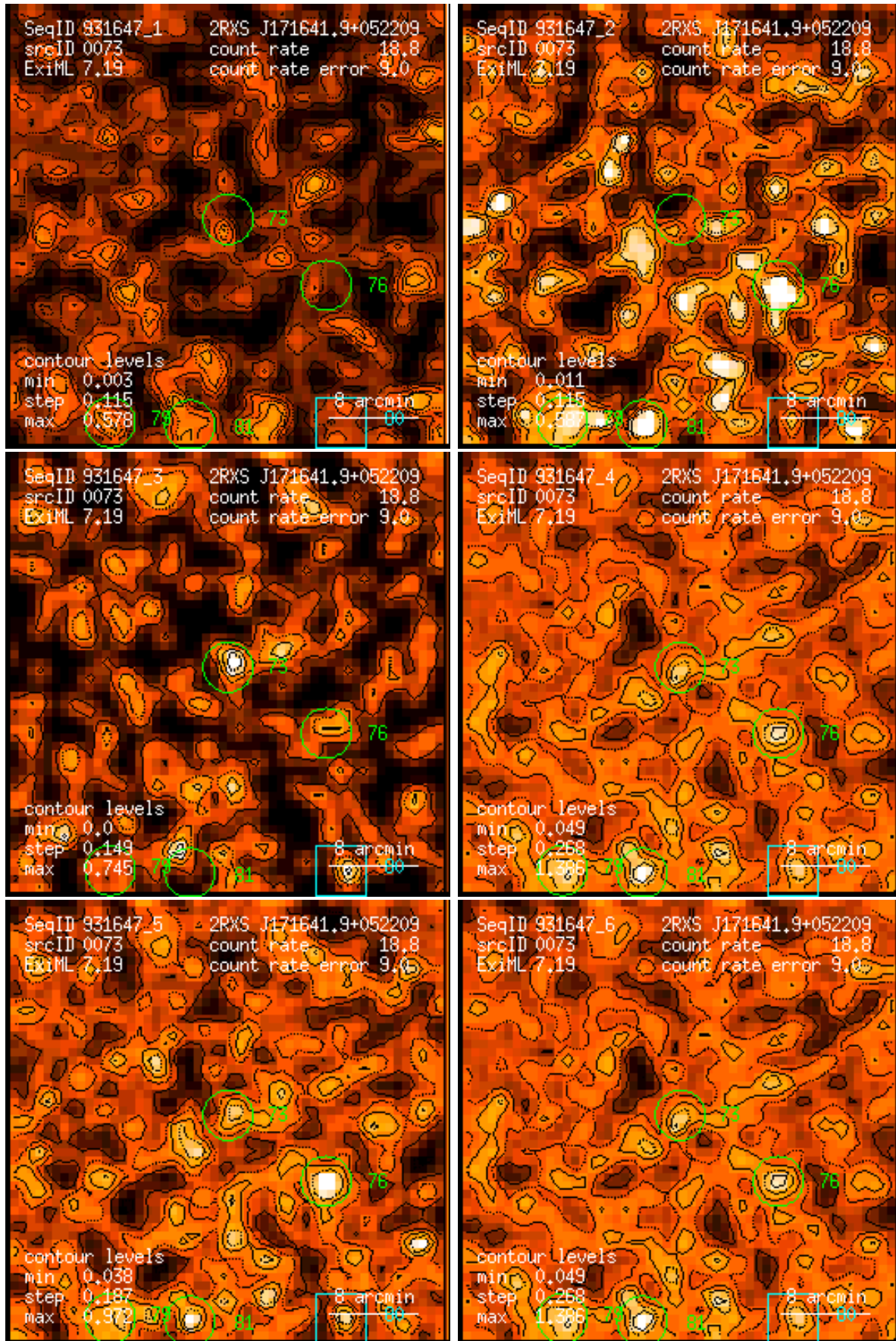
Figure 73: RASS 931647: detection 0073: band rate images, Gaussian filter: (1) PSPC channels 11 – 41, (2) 52 – 90, (3) 91 – 201, (4) 11 – 235, (5) 52 – 201, (6) 11 – 201. Broad band rates in counts/ks. Band rate contour levels in counts/ks/arcmin 2 .
