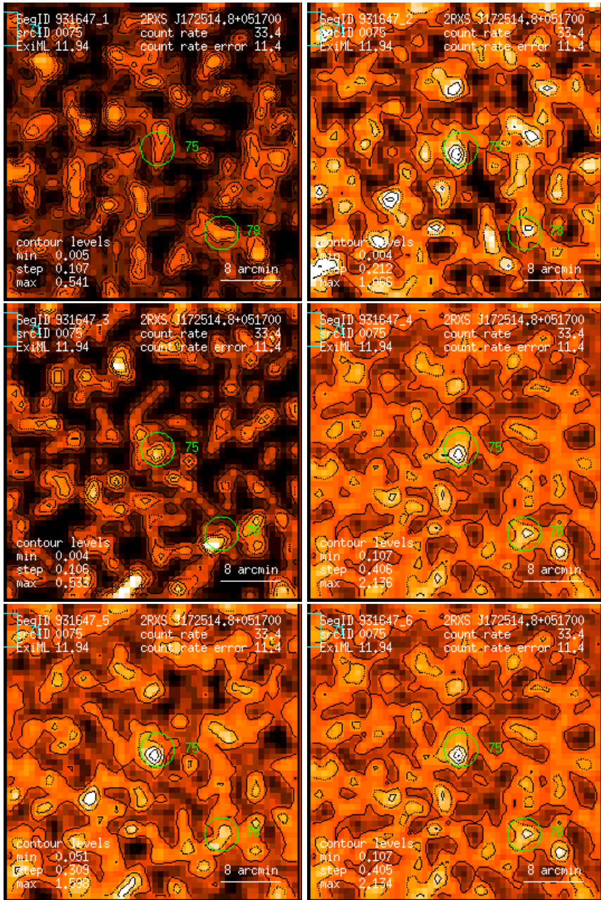
Figure 75: RASS 931647: detection 0075: band rate images, Gaussian filter: (1) PSPC channels 11 – 41, (2) 52 – 90, (3) 91 – 201, (4) 11 – 235, (5) 52 – 201, (6) 11 – 201. Broad band rates in counts/ks. Band rate contour levels in counts/ks/arcmin 2 .
