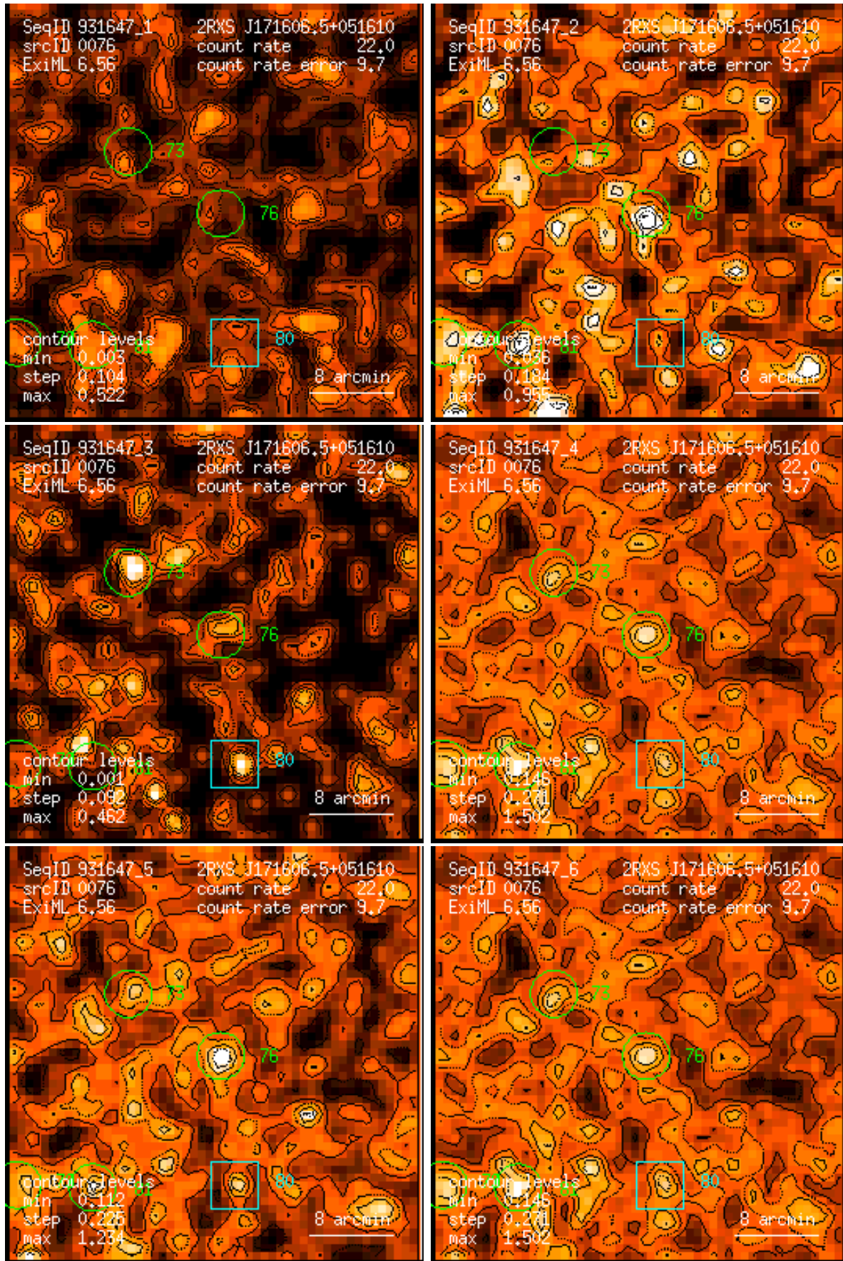
Figure 76: RASS 931647: detection 0076: band rate images, Gaussian filter: (1) PSPC channels 11 – 41, (2) 52 – 90, (3) 91 – 201, (4) 11 – 235, (5) 52 – 201, (6) 11 – 201. Broad band rates in counts/ks. Band rate contour levels in counts/ks/arcmin 2 .
