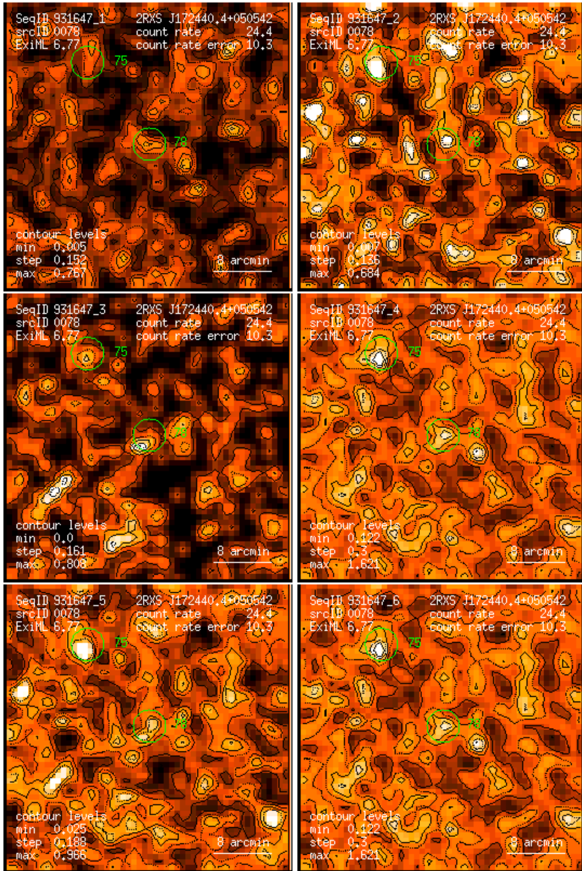
Figure 78: RASS 931647: detection 0078: band rate images, Gaussian filter: (1) PSPC channels 11 – 41, (2) 52 – 90, (3) 91 – 201, (4) 11 – 235, (5) 52 – 201, (6) 11 – 201. Broad band rates in counts/ks. Band rate contour levels in counts/ks/arcmin 2 .
