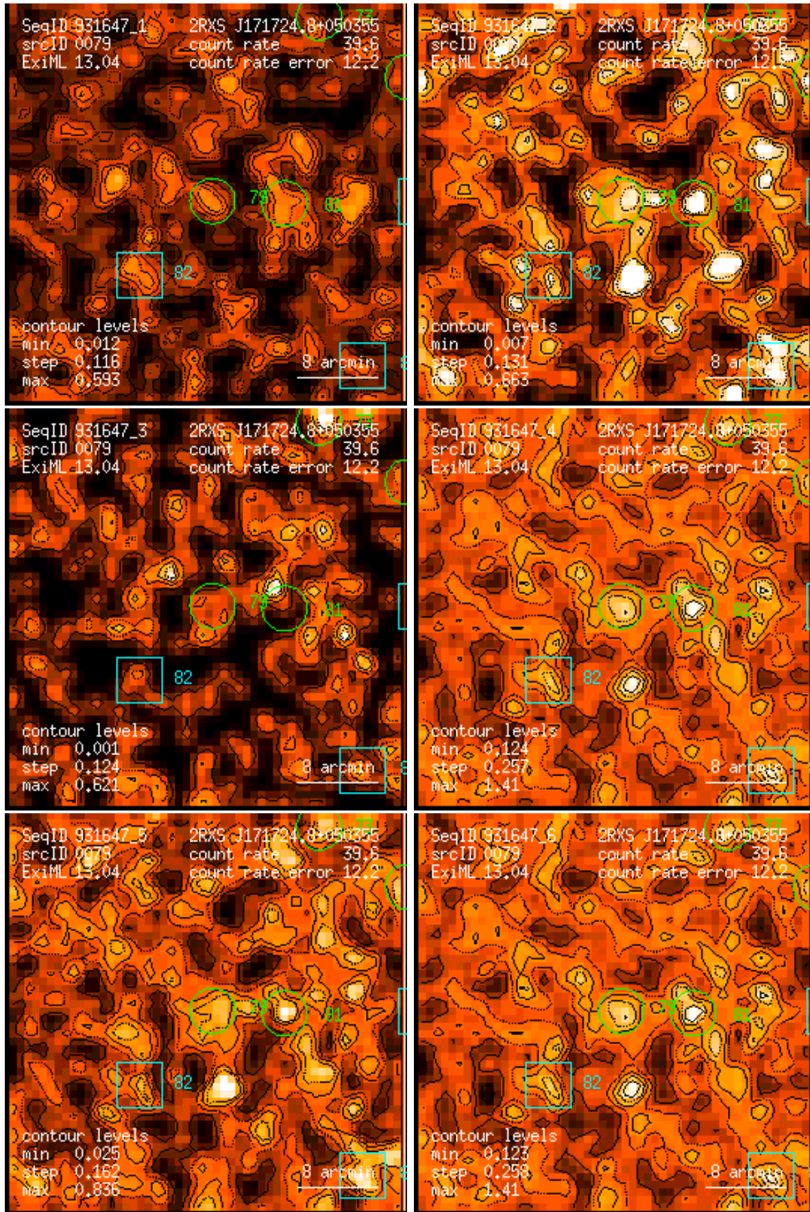
Figure 79: RASS 931647: detection 0079: band rate images, Gaussian filter: (1) PSPC channels 11 – 41, (2) 52 – 90, (3) 91 – 201, (4) 11 – 235, (5) 52 – 201, (6) 11 – 201. Broad band rates in counts/ks. Band rate contour levels in counts/ks/arcmin 2 .
