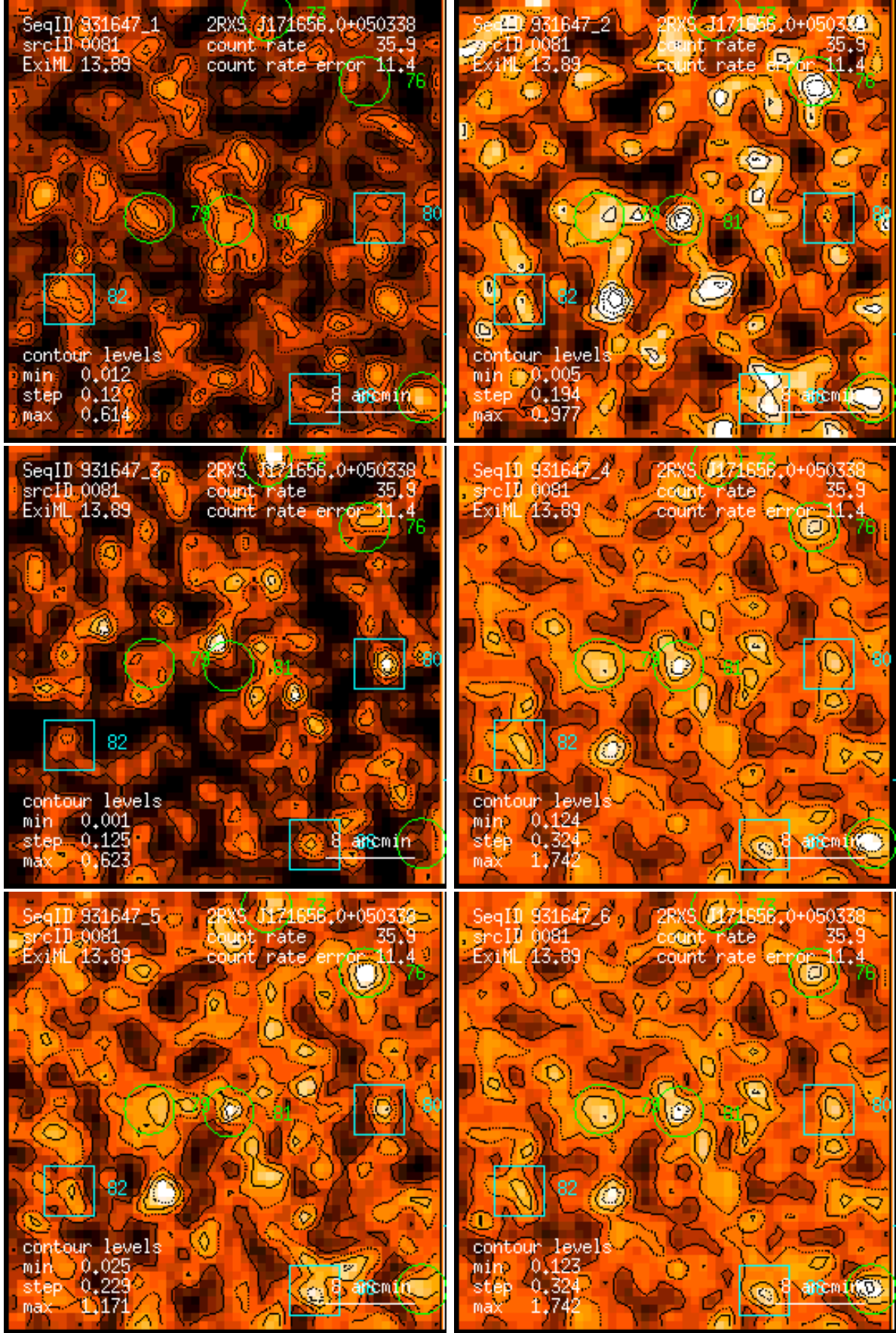
Figure 81: RASS 931647: detection 0081: band rate images, Gaussian filter: (1) PSPC channels 11 – 41, (2) 52 – 90, (3) 91 – 201, (4) 11 – 235, (5) 52 – 201, (6) 11 – 201. Broad band rates in counts/ks. Band rate contour levels in counts/ks/arcmin 2 .
