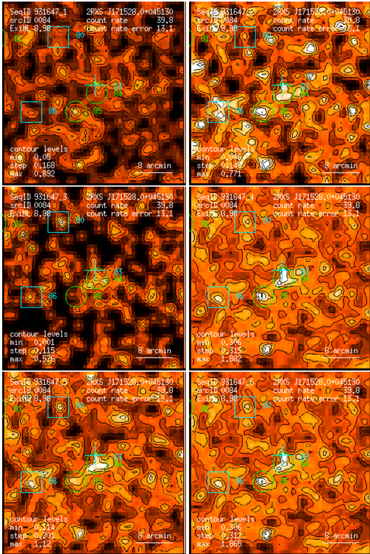
Figure 84: RASS 931647: detection 0084: band rate images, Gaussian filter: (1) PSPC channels 11 – 41, (2) 52 – 90, (3) 91 – 201, (4) 11 – 235, (5) 52 – 201, (6) 11 – 201. Broad band rates in counts/ks. Band rate contour levels in counts/ks/arcmin 2 .
