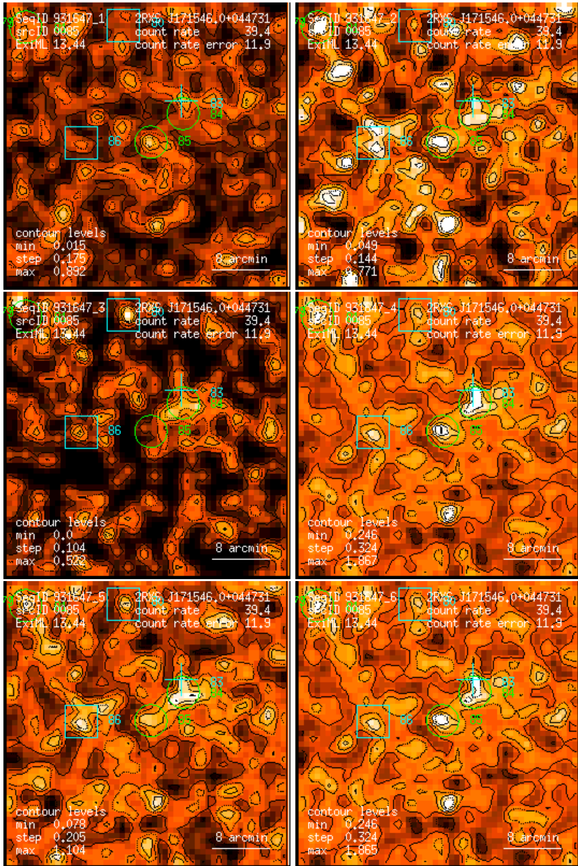
Figure 85: RASS 931647: detection 0085: band rate images, Gaussian filter: (1) PSPC channels 11 – 41, (2) 52 – 90, (3) 91 – 201, (4) 11 – 235, (5) 52 – 201, (6) 11 – 201. Broad band rates in counts/ks. Band rate contour levels in counts/ks/arcmin 2 .
