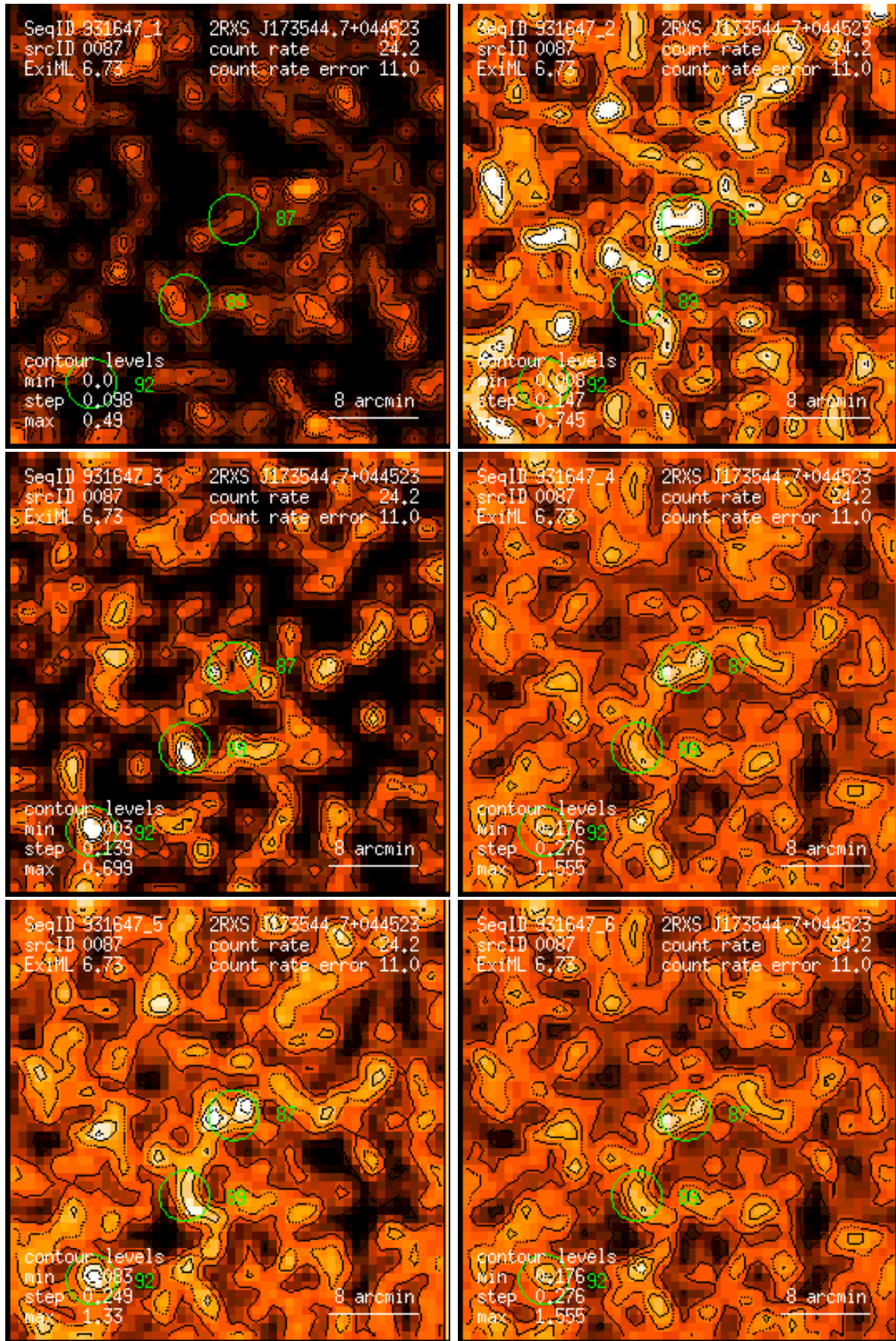
Figure 87: RASS 931647: detection 0087: band rate images, Gaussian filter: (1) PSPC channels 11 – 41, (2) 52 – 90, (3) 91 – 201, (4) 11 – 235, (5) 52 – 201, (6) 11 – 201. Broad band rates in counts/ks. Band rate contour levels in counts/ks/arcmin 2 .
