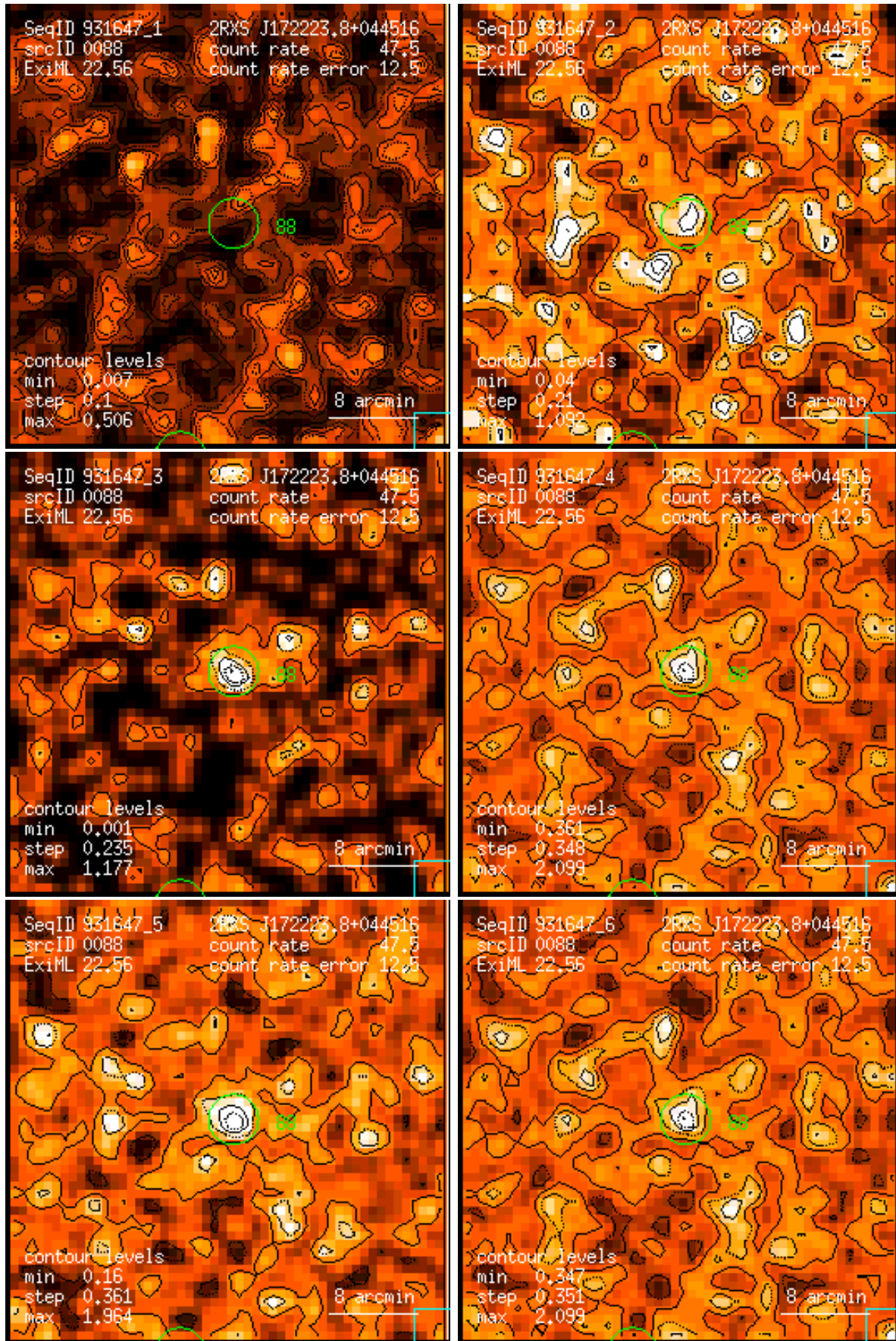
Figure 88: RASS 931647: detection 0088: band rate images, Gaussian filter: (1) PSPC channels 11 – 41, (2) 52 – 90, (3) 91 – 201, (4) 11 – 235, (5) 52 – 201, (6) 11 – 201. Broad band rates in counts/ks. Band rate contour levels in counts/ks/arcmin 2 .
