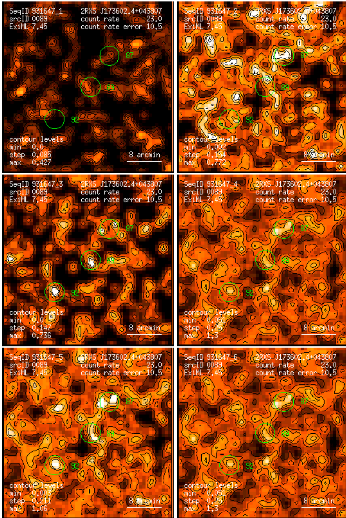
Figure 89: RASS 931647: detection 0089: band rate images, Gaussian filter: (1) PSPC channels 11 – 41, (2) 52 – 90, (3) 91 – 201, (4) 11 – 235, (5) 52 – 201, (6) 11 – 201. Broad band rates in counts/ks. Band rate contour levels in counts/ks/arcmin 2 .
