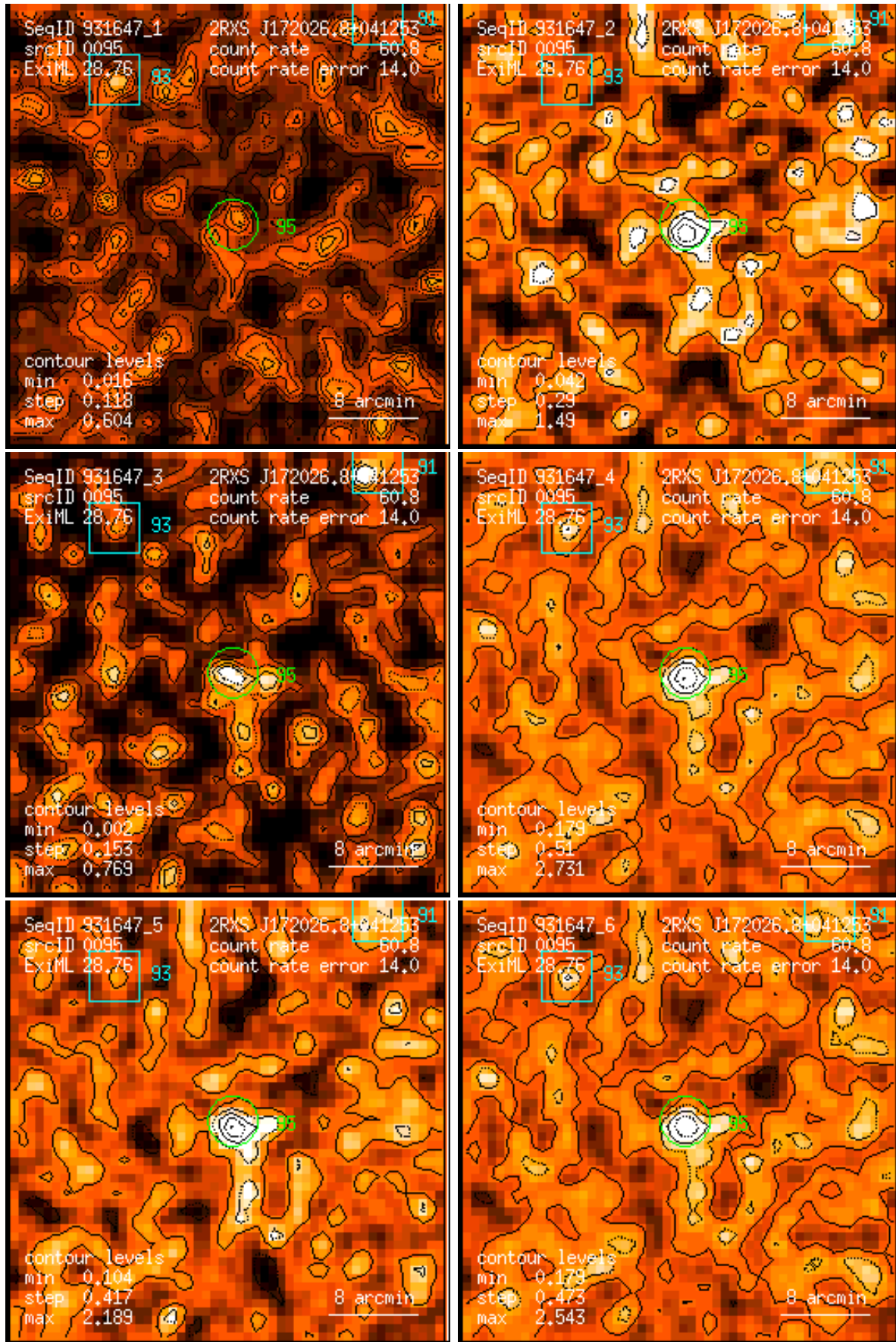
Figure 95: RASS 931647: detection 0095: band rate images, Gaussian filter: (1) PSPC channels 11 – 41, (2) 52 – 90, (3) 91 – 201, (4) 11 – 235, (5) 52 – 201, (6) 11 – 201. Broad band rates in counts/ks. Band rate contour levels in counts/ks/arcmin 2 .
