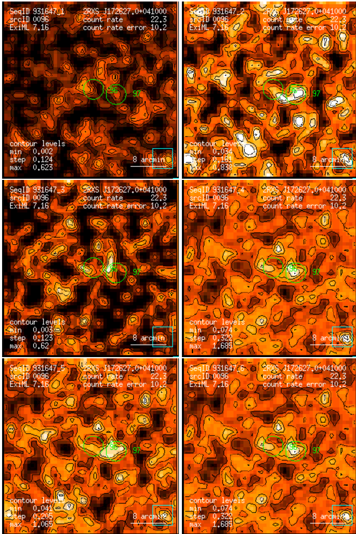
Figure 96: RASS 931647: detection 0096: band rate images, Gaussian filter: (1) PSPC channels 11 – 41, (2) 52 – 90, (3) 91 – 201, (4) 11 – 235, (5) 52 – 201, (6) 11 – 201. Broad band rates in counts/ks. Band rate contour levels in counts/ks/arcmin 2 .
