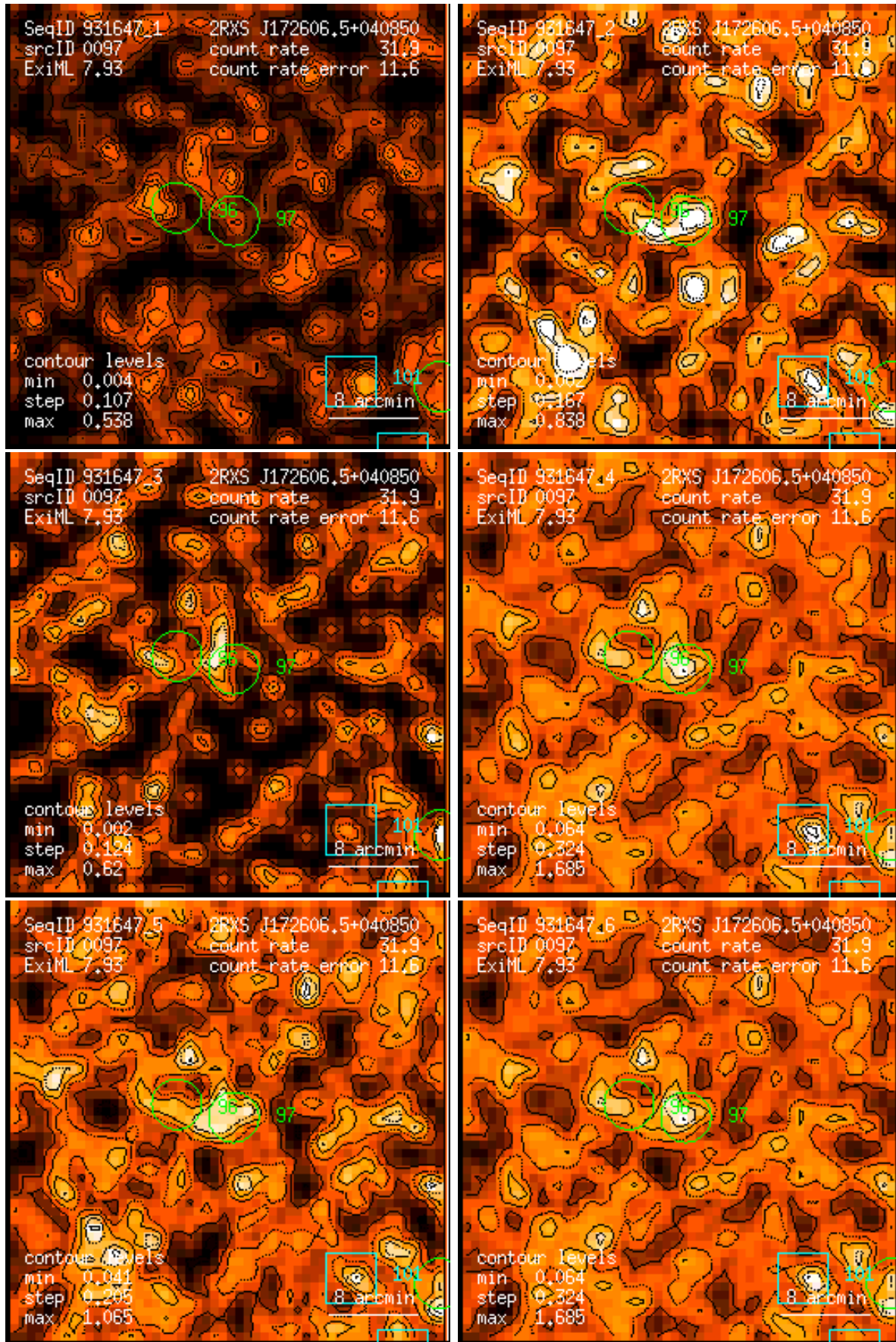
Figure 97: RASS 931647: detection 0097: band rate images, Gaussian filter: (1) PSPC channels 11 – 41, (2) 52 – 90, (3) 91 – 201, (4) 11 – 235, (5) 52 – 201, (6) 11 – 201. Broad band rates in counts/ks. Band rate contour levels in counts/ks/arcmin 2 .
