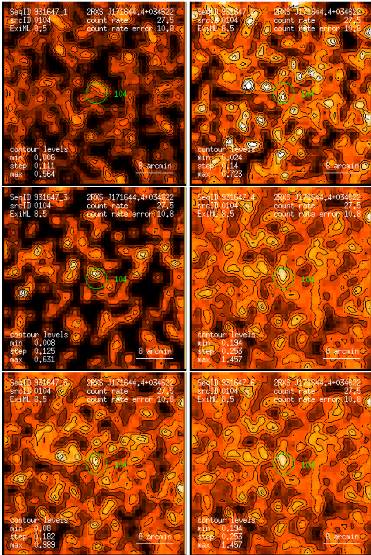
Figure 104: RASS 931647: detection 0104: band rate images, Gaussian filter: (1) PSPC channels 11 – 41, (2) 52 – 90, (3) 91 – 201, (4) 11 – 235, (5) 52 – 201, (6) 11 – 201. Broad band rates in counts/ks. Band rate contour levels in counts/ks/arcmin 2 .
