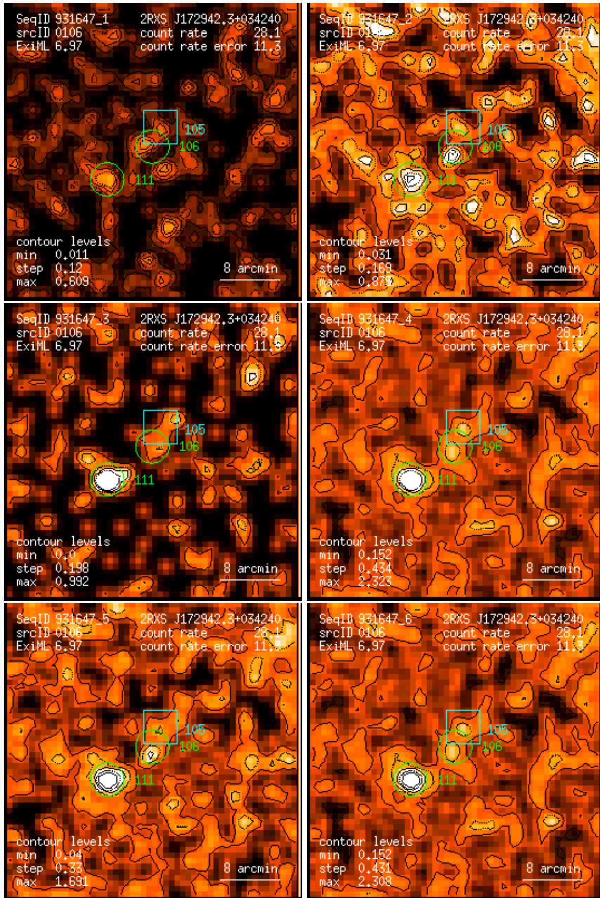
Figure 106: RASS 931647: detection 0106: band rate images, Gaussian filter: (1) PSPC channels 11 – 41, (2) 52 – 90, (3) 91 – 201, (4) 11 – 235, (5) 52 – 201, (6) 11 – 201. Broad band rates in counts/ks. Band rate contour levels in counts/ks/arcmin 2 .
