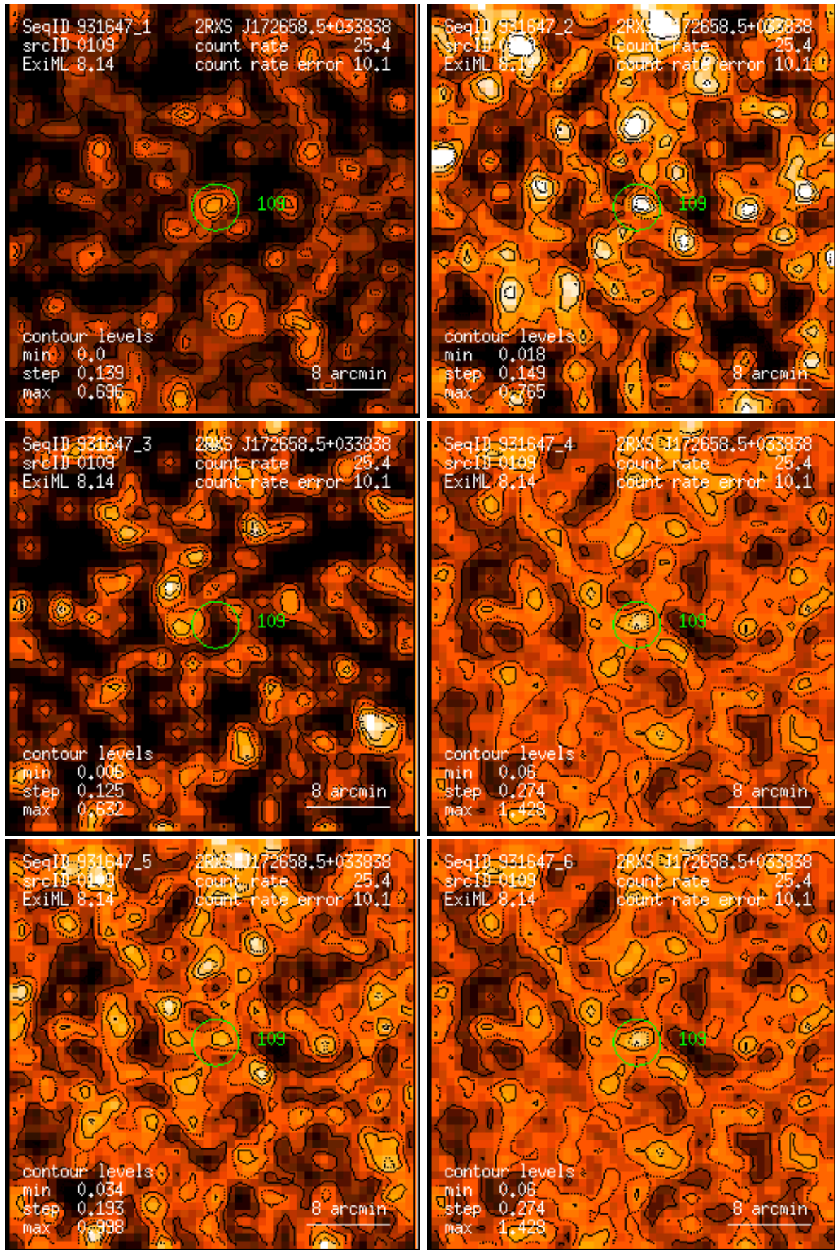
Figure 109: RASS 931647: detection 0109: band rate images, Gaussian filter: (1) PSPC channels 11 – 41, (2) 52 – 90, (3) 91 – 201, (4) 11 – 235, (5) 52 – 201, (6) 11 – 201. Broad band rates in counts/ks. Band rate contour levels in counts/ks/arcmin 2 .
