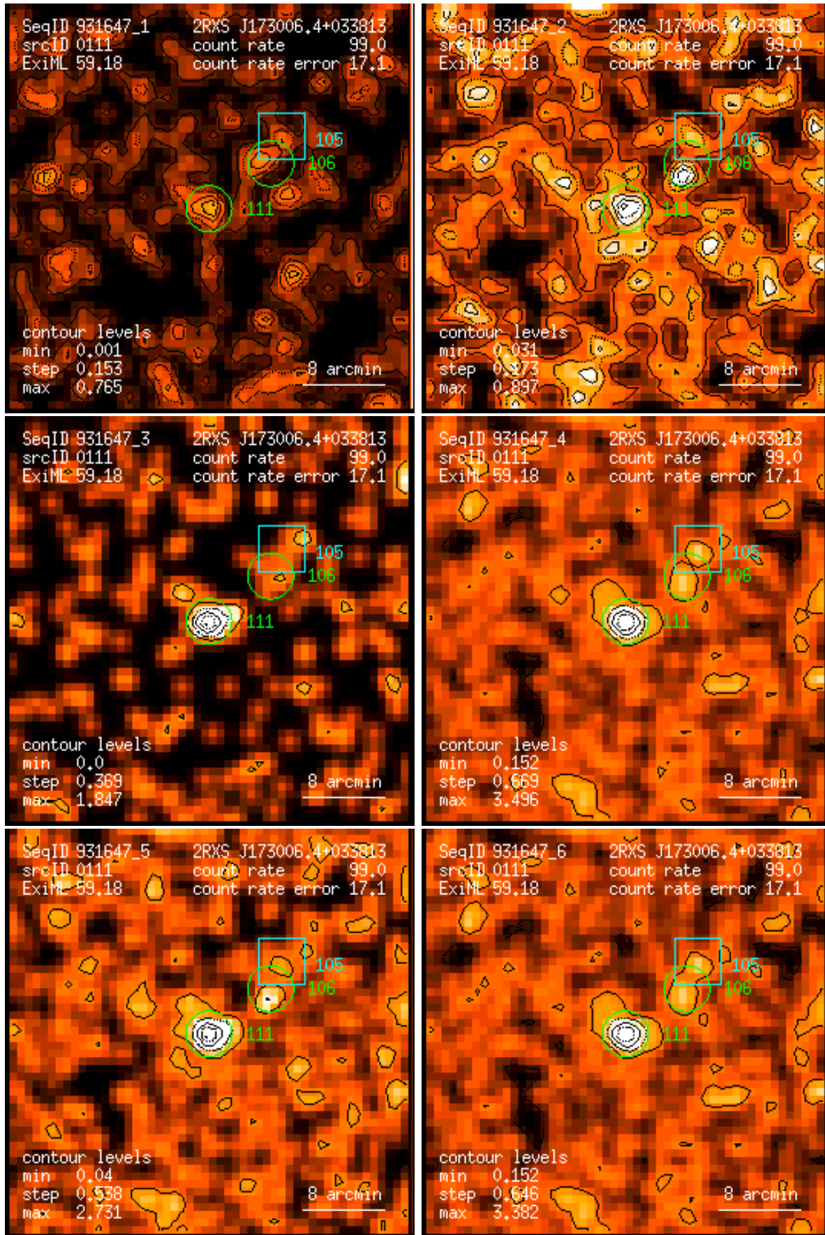
Figure 111: RASS 931647: detection 0111: band rate images, Gaussian filter: (1) PSPC channels 11 – 41, (2) 52 – 90, (3) 91 – 201, (4) 11 – 235, (5) 52 – 201, (6) 11 – 201. Broad band rates in counts/ks. Band rate contour levels in counts/ks/arcmin 2 .
