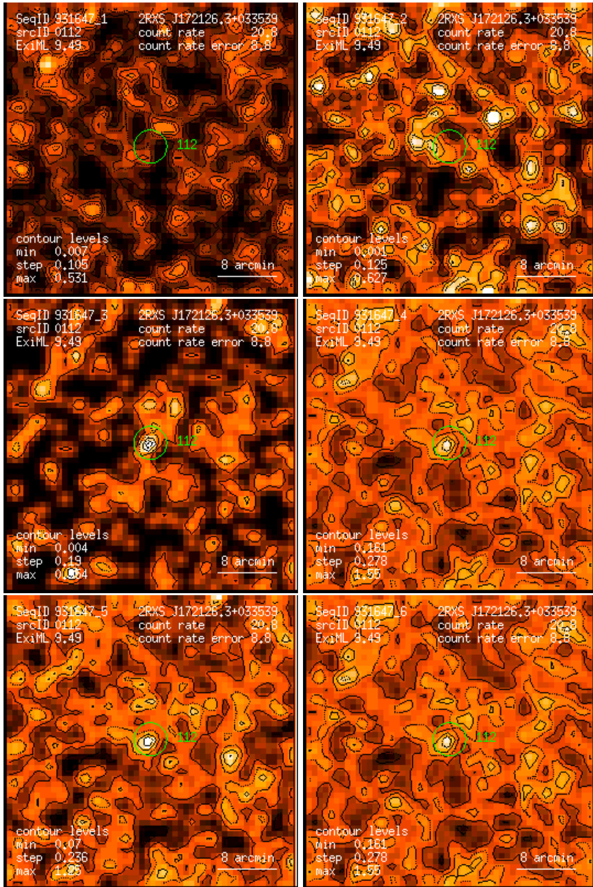
Figure 112: RASS 931647: detection 0112: band rate images, Gaussian filter: (1) PSPC channels 11 – 41, (2) 52 – 90, (3) 91 – 201, (4) 11 – 235, (5) 52 – 201, (6) 11 – 201. Broad band rates in counts/ks. Band rate contour levels in counts/ks/arcmin 2 .
