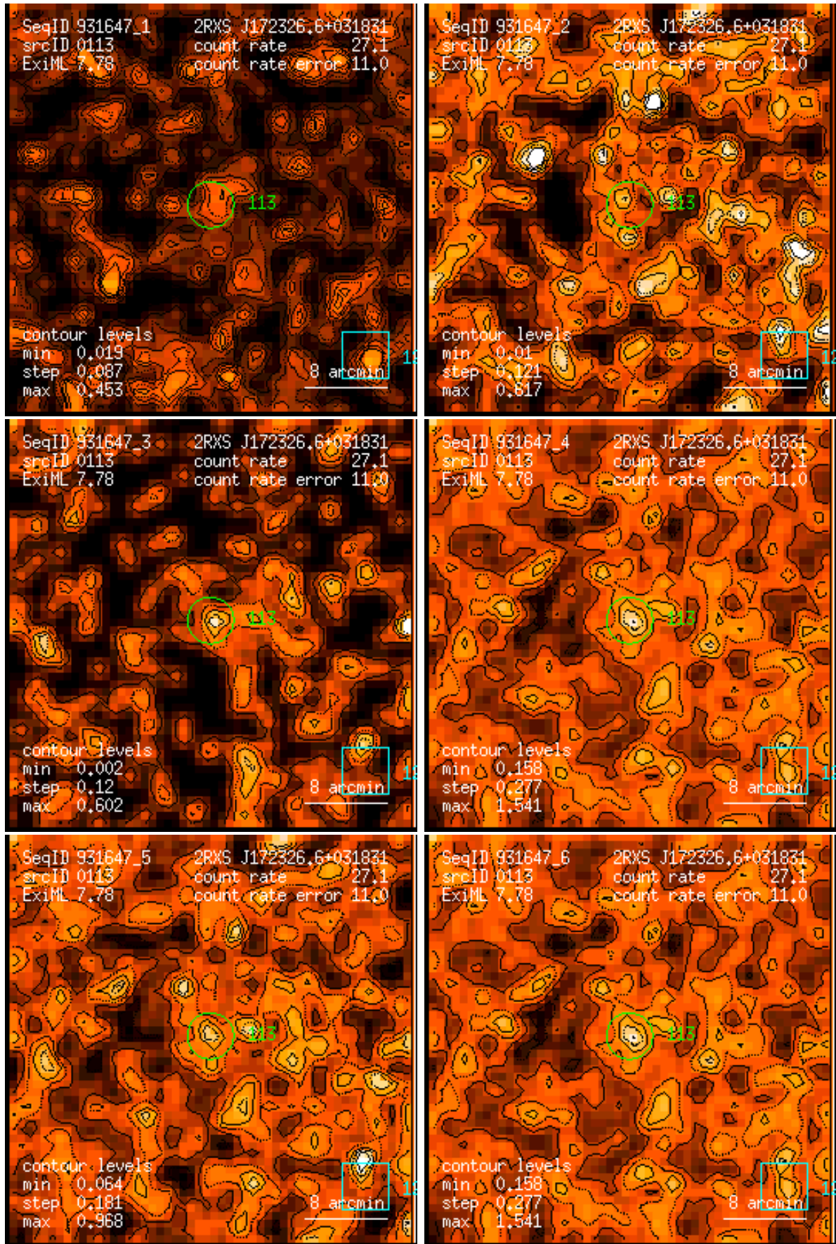
Figure 113: RASS 931647: detection 0113: band rate images, Gaussian filter: (1) PSPC channels 11 – 41, (2) 52 – 90, (3) 91 – 201, (4) 11 – 235, (5) 52 – 201, (6) 11 – 201. Broad band rates in counts/ks. Band rate contour levels in counts/ks/arcmin 2 .
