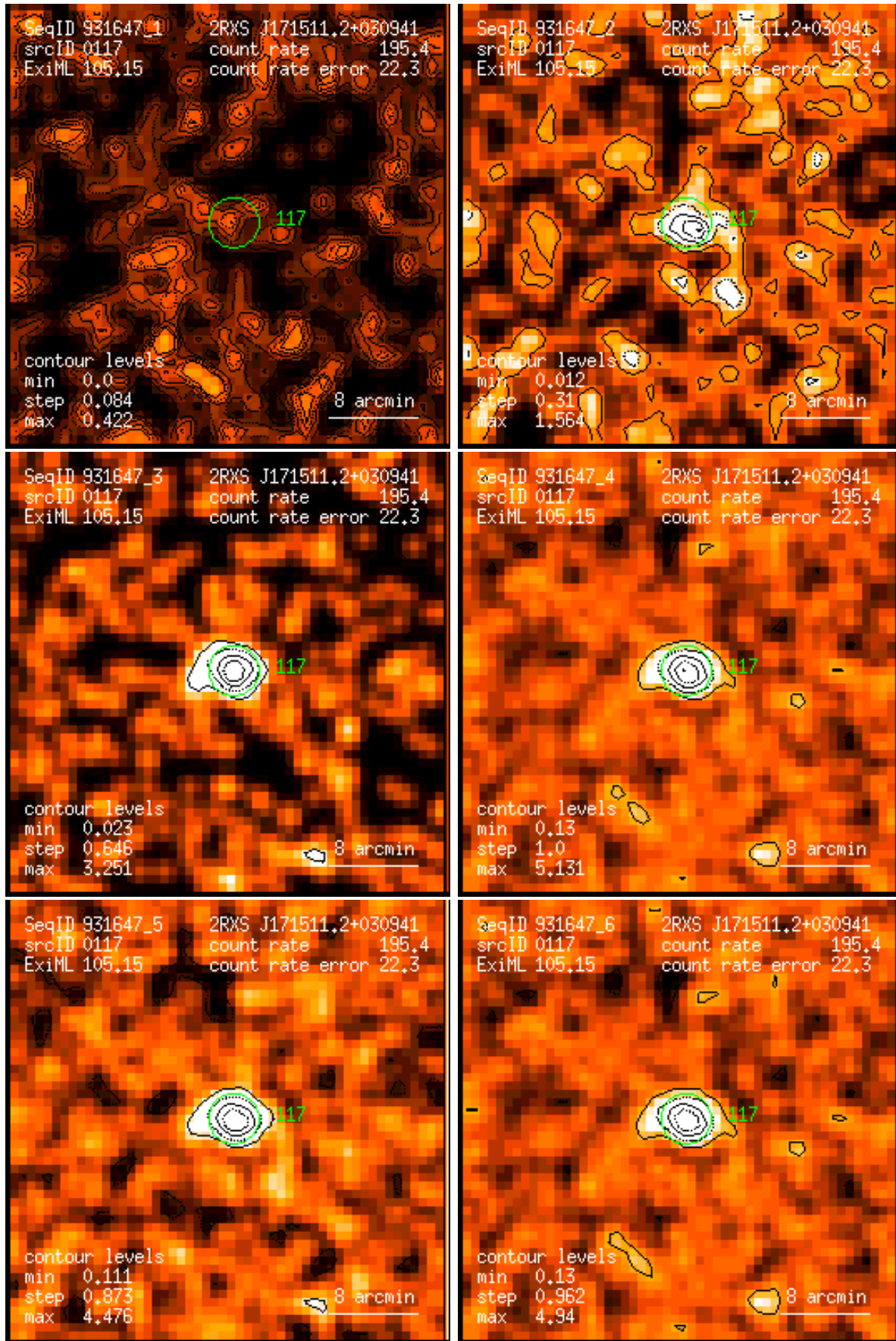
Figure 117: RASS 931647: detection 0117: band rate images, Gaussian filter: (1) PSPC channels 11 – 41, (2) 52 – 90, (3) 91 – 201, (4) 11 – 235, (5) 52 – 201, (6) 11 – 201. Broad band rates in counts/ks. Band rate contour levels in counts/ks/arcmin 2 .
