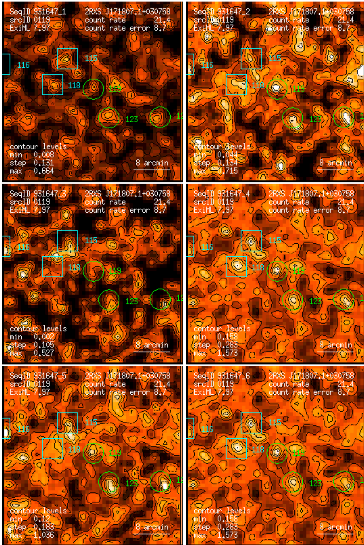
Figure 119: RASS 931647: detection 0119: band rate images, Gaussian filter: (1) PSPC channels 11 – 41, (2) 52 – 90, (3) 91 – 201, (4) 11 – 235, (5) 52 – 201, (6) 11 – 201. Broad band rates in counts/ks. Band rate contour levels in counts/ks/arcmin 2 .
