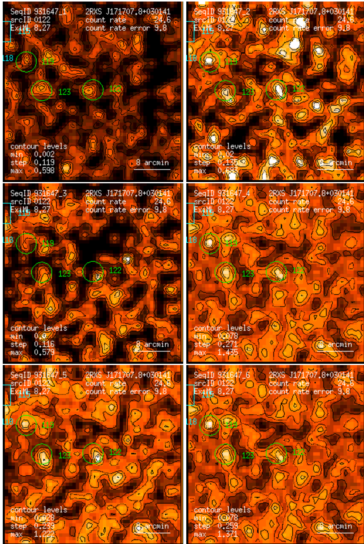
Figure 122: RASS 931647: detection 0122: band rate images, Gaussian filter: (1) PSPC channels 11 – 41, (2) 52 – 90, (3) 91 – 201, (4) 11 – 235, (5) 52 – 201, (6) 11 – 201. Broad band rates in counts/ks. Band rate contour levels in counts/ks/arcmin 2 .
