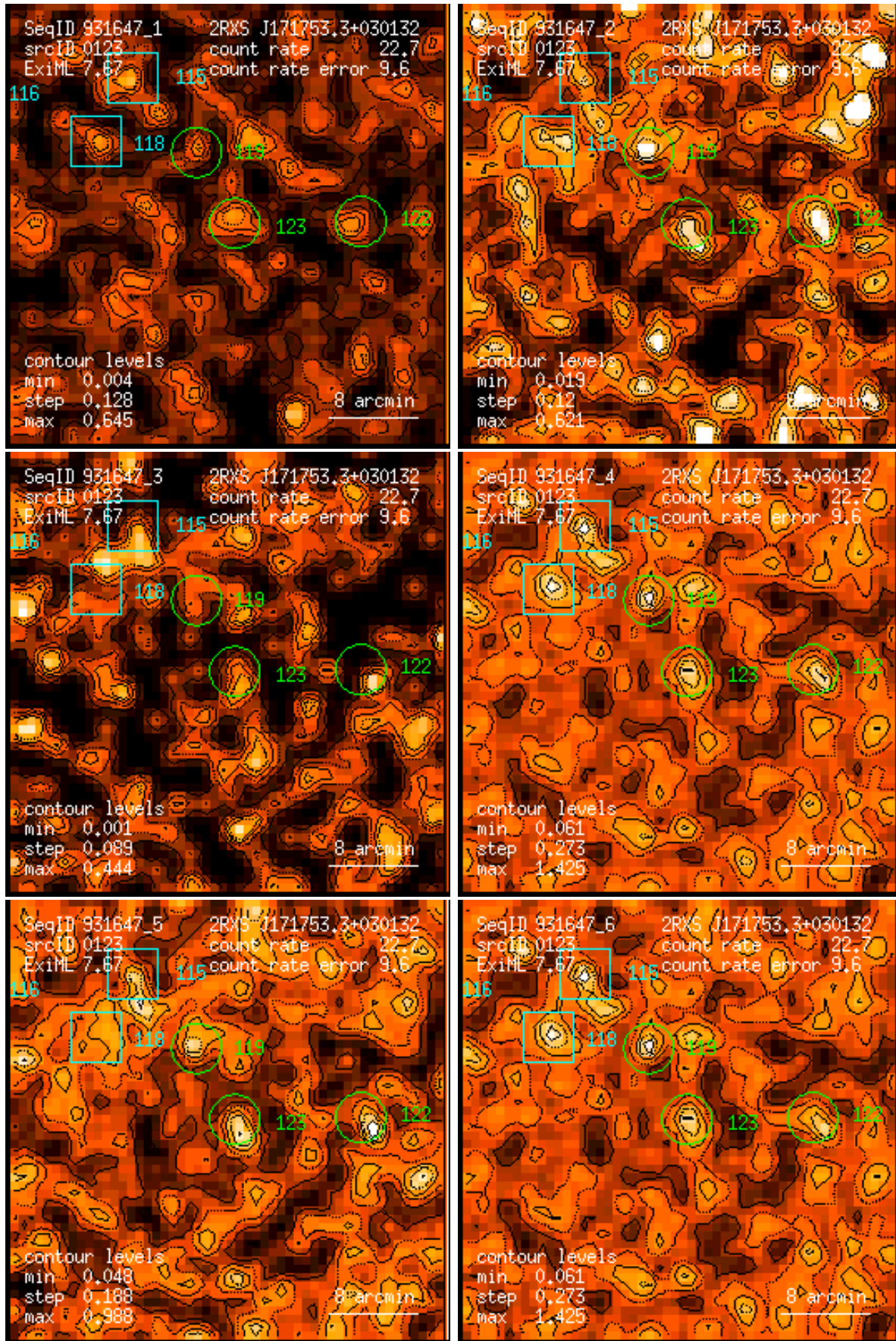
Figure 123: RASS 931647: detection 0123: band rate images, Gaussian filter: (1) PSPC channels 11 – 41, (2) 52 – 90, (3) 91 – 201, (4) 11 – 235, (5) 52 – 201, (6) 11 – 201. Broad band rates in counts/ks. Band rate contour levels in counts/ks/arcmin 2 .
