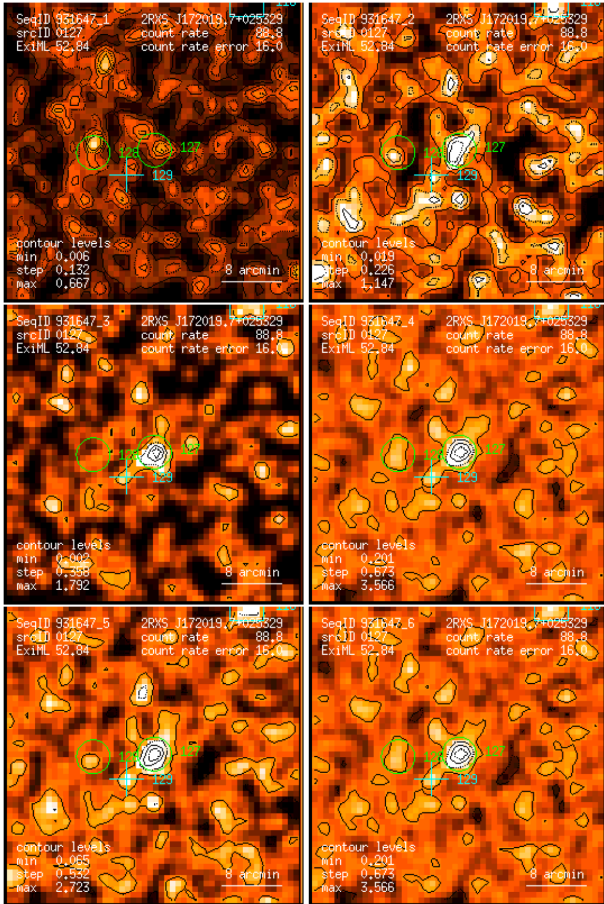
Figure 127: RASS 931647: detection 0127: band rate images, Gaussian filter: (1) PSPC channels 11 – 41, (2) 52 – 90, (3) 91 – 201, (4) 11 – 235, (5) 52 – 201, (6) 11 – 201. Broad band rates in counts/ks. Band rate contour levels in counts/ks/arcmin 2 .
