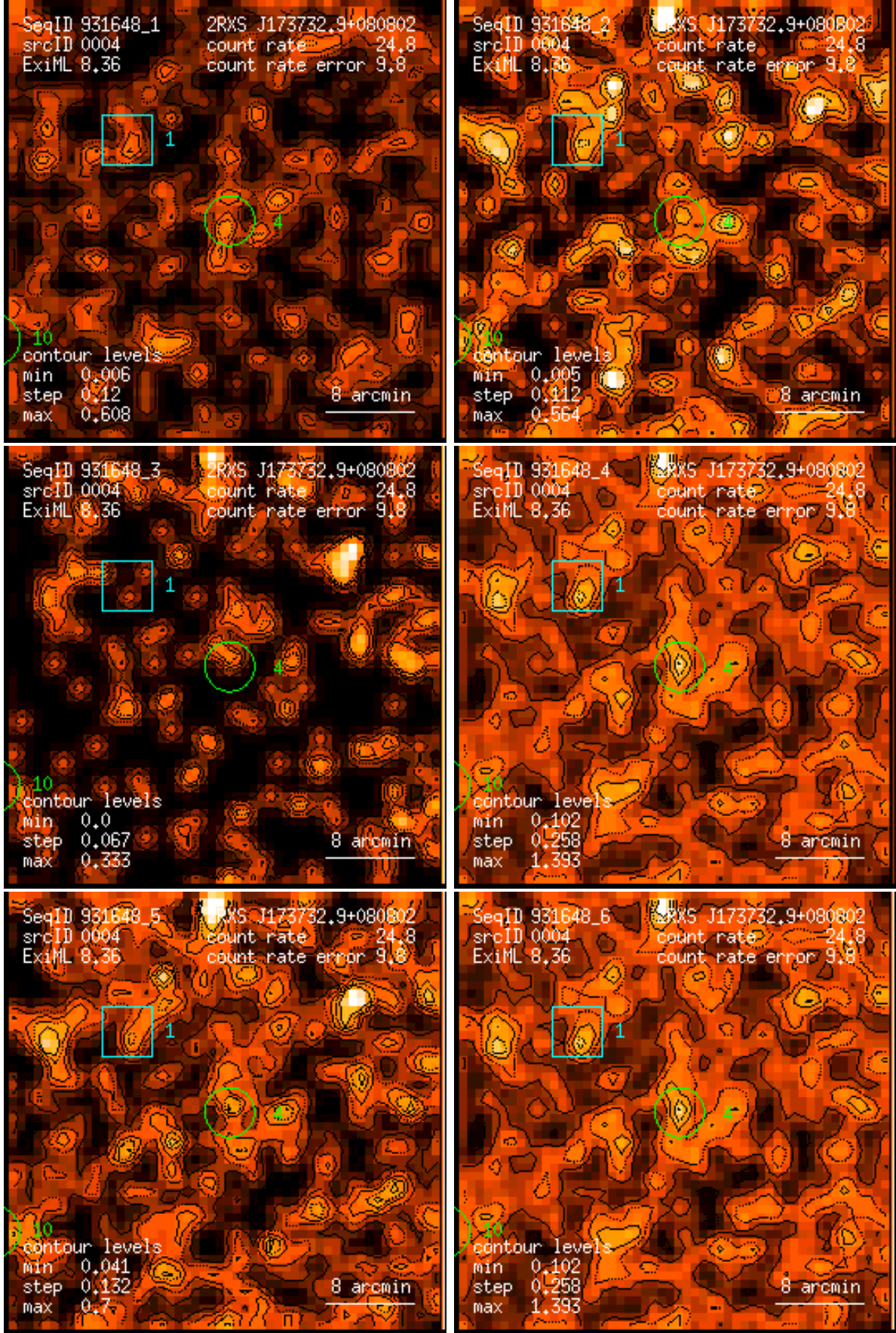
Figure 4: RASS 931648: detection 0004: band rate images, Gaussian filter: (1) PSPC channels 11 – 41, (2) 52 – 90, (3) 91 – 201, (4) 11 – 235, (5) 52 – 201, (6) 11 – 201. Broad band rates in counts/ks. Band rate contour levels in counts/ks/arcmin 2 .
