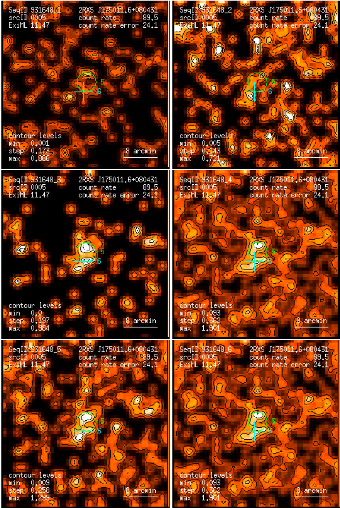
Figure 5: RASS 931648: detection 0005: band rate images, Gaussian filter: (1) PSPC channels 11 – 41, (2) 52 – 90, (3) 91 – 201, (4) 11 – 235, (5) 52 – 201, (6) 11 – 201. Broad band rates in counts/ks. Band rate contour levels in counts/ks/arcmin 2 .
