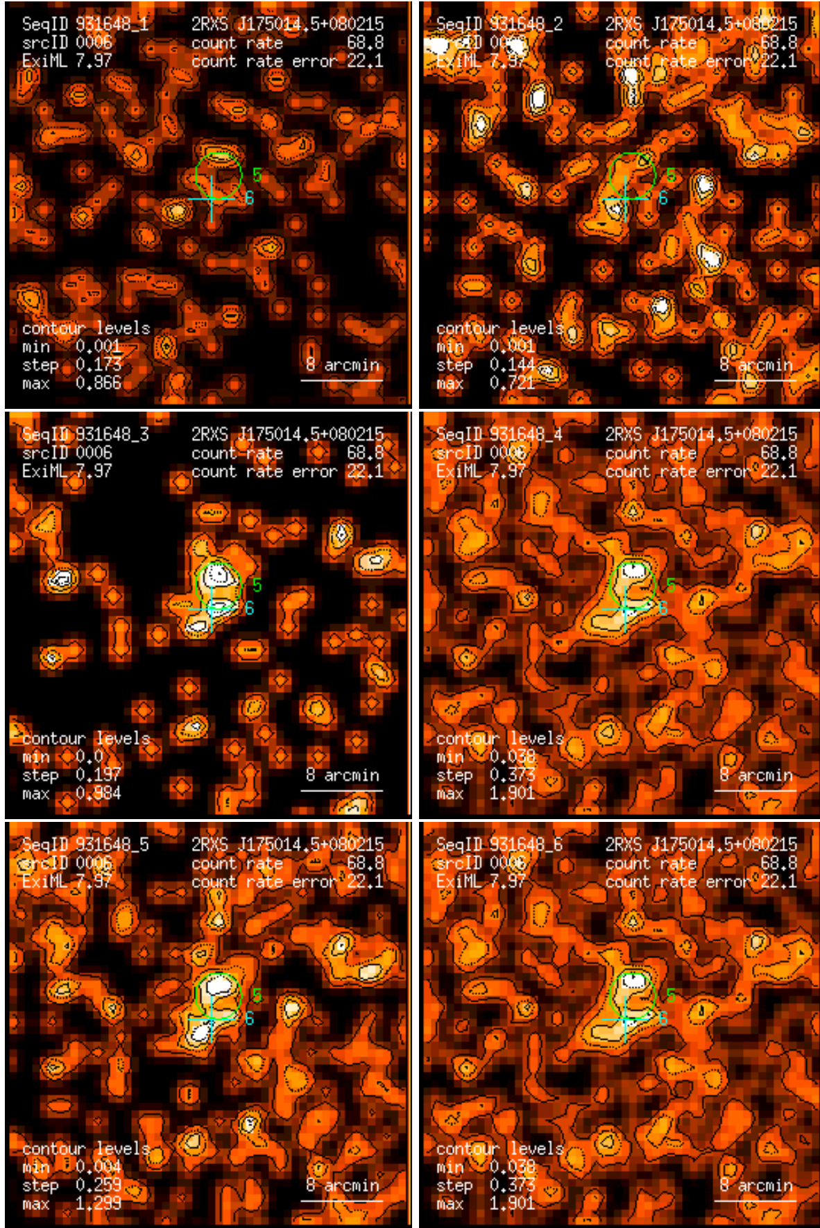
Figure 6: RASS 931648: detection 0006: band rate images, Gaussian filter: (1) PSPC channels 11 – 41, (2) 52 – 90, (3) 91 – 201, (4) 11 – 235, (5) 52 – 201, (6) 11 – 201. Broad band rates in counts/ks. Band rate contour levels in counts/ks/arcmin 2 .
