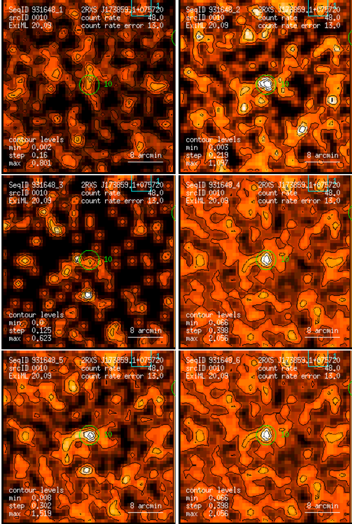
Figure 10: RASS 931648: detection 0010: band rate images, Gaussian filter: (1) PSPC channels 11 – 41, (2) 52 – 90, (3) 91 – 201, (4) 11 – 235, (5) 52 – 201, (6) 11 – 201. Broad band rates in counts/ks. Band rate contour levels in counts/ks/arcmin 2 .
