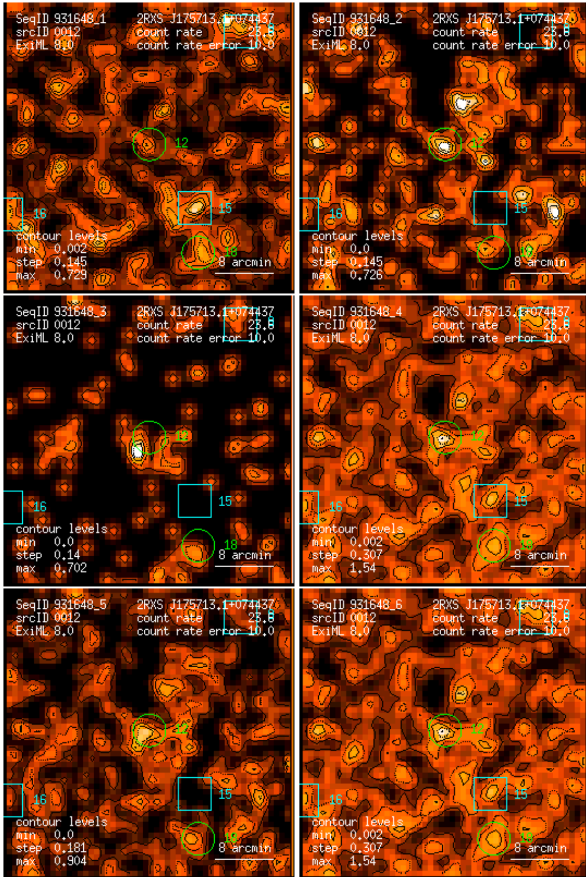
Figure 12: RASS 931648: detection 0012: band rate images, Gaussian filter: (1) PSPC channels 11 – 41, (2) 52 – 90, (3) 91 – 201, (4) 11 – 235, (5) 52 – 201, (6) 11 – 201. Broad band rates in counts/ks. Band rate contour levels in counts/ks/arcmin 2 .
