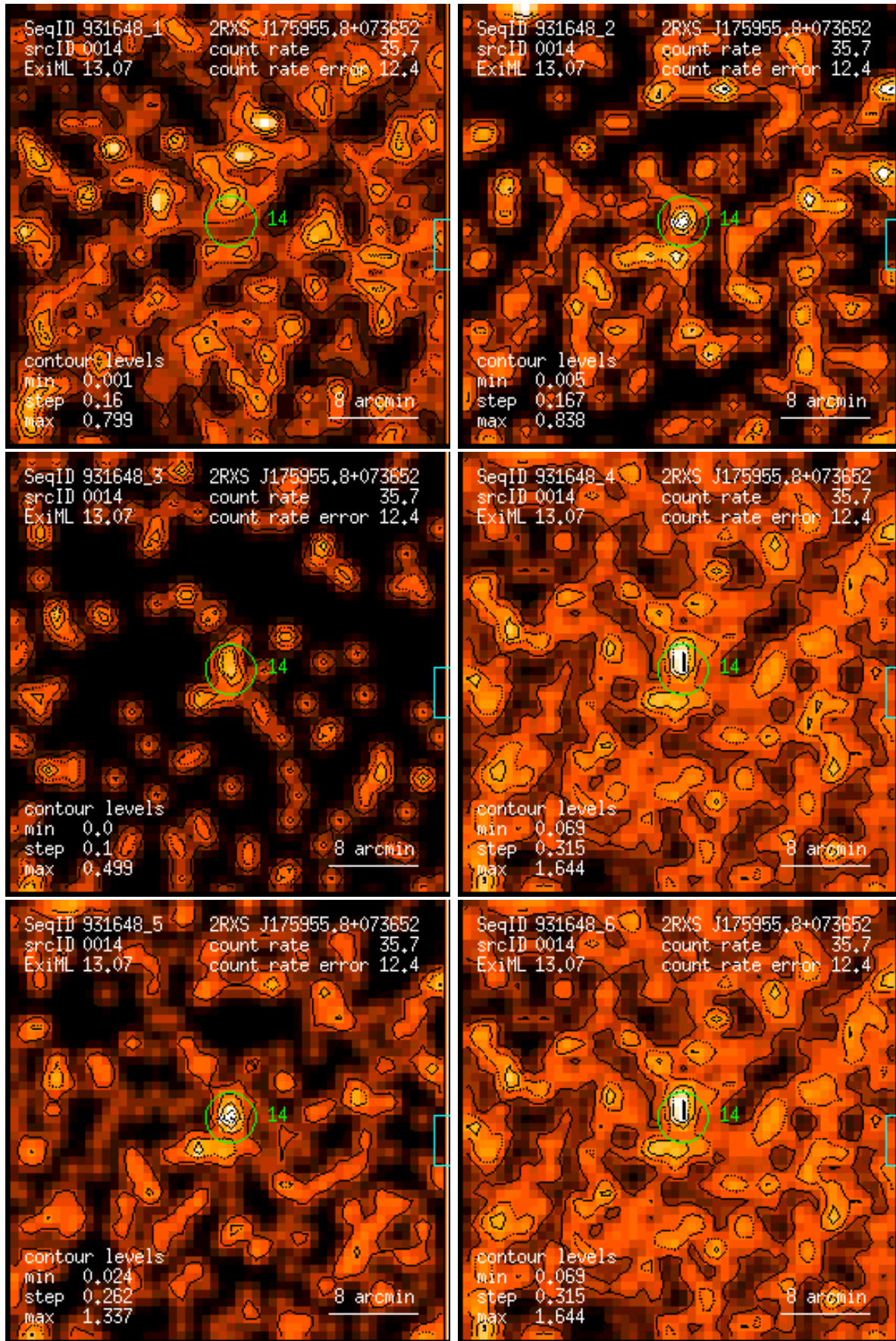
Figure 14: RASS 931648: detection 0014: band rate images, Gaussian filter: (1) PSPC channels 11 – 41, (2) 52 – 90, (3) 91 – 201, (4) 11 – 235, (5) 52 – 201, (6) 11 – 201. Broad band rates in counts/ks. Band rate contour levels in counts/ks/arcmin 2 .
