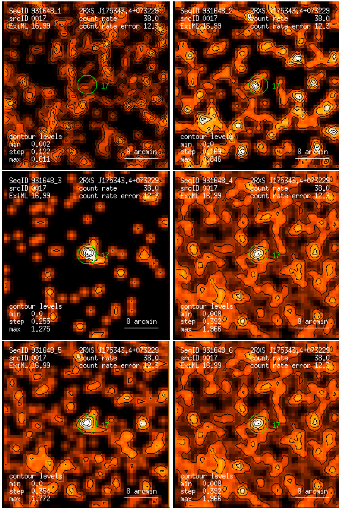
Figure 17: RASS 931648: detection 0017: band rate images, Gaussian filter: (1) PSPC channels 11 – 41, (2) 52 – 90, (3) 91 – 201, (4) 11 – 235, (5) 52 – 201, (6) 11 – 201. Broad band rates in counts/ks. Band rate contour levels in counts/ks/arcmin 2 .
