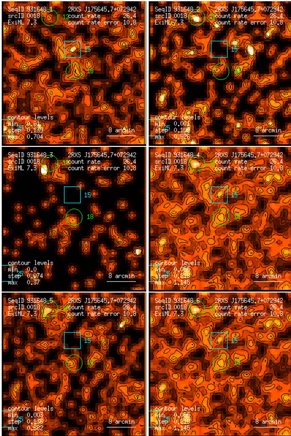
Figure 18: RASS 931648: detection 0018: band rate images, Gaussian filter: (1) PSPC channels 11 – 41, (2) 52 – 90, (3) 91 – 201, (4) 11 – 235, (5) 52 – 201, (6) 11 – 201. Broad band rates in counts/ks. Band rate contour levels in counts/ks/arcmin 2 .
