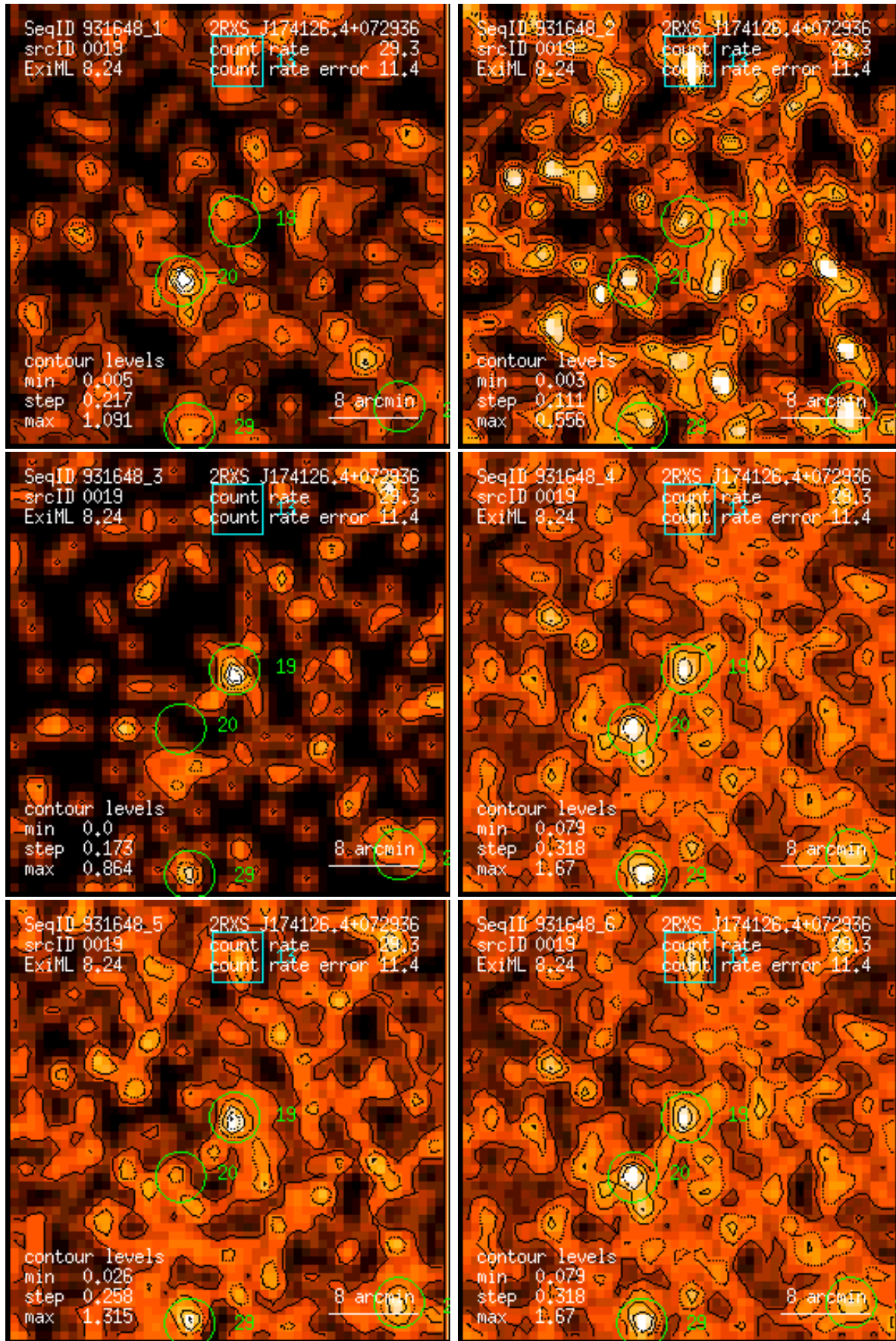
Figure 19: RASS 931648: detection 0019: band rate images, Gaussian filter: (1) PSPC channels 11 – 41, (2) 52 – 90, (3) 91 – 201, (4) 11 – 235, (5) 52 – 201, (6) 11 – 201. Broad band rates in counts/ks. Band rate contour levels in counts/ks/arcmin 2 .
