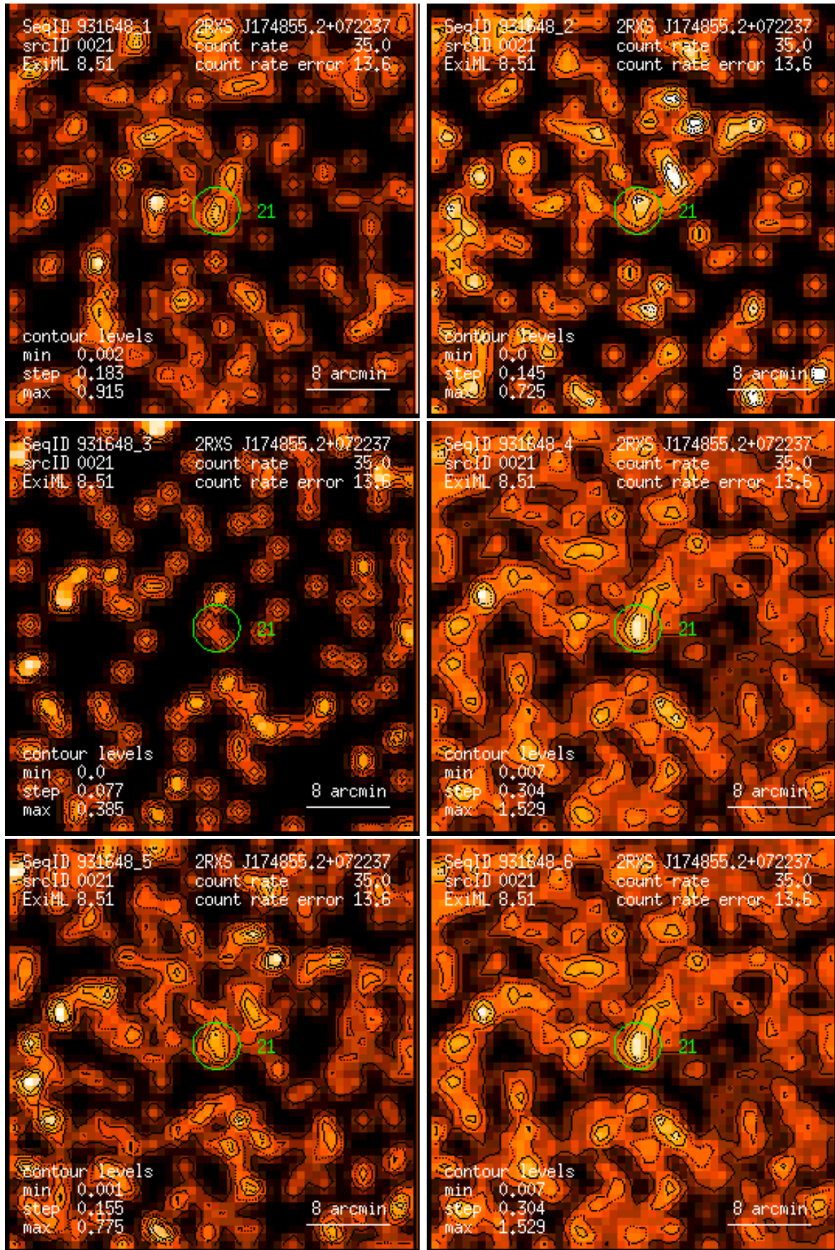
Figure 21: RASS 931648: detection 0021: band rate images, Gaussian filter: (1) PSPC channels 11 – 41, (2) 52 – 90, (3) 91 – 201, (4) 11 – 235, (5) 52 – 201, (6) 11 – 201. Broad band rates in counts/ks. Band rate contour levels in counts/ks/arcmin 2 .
