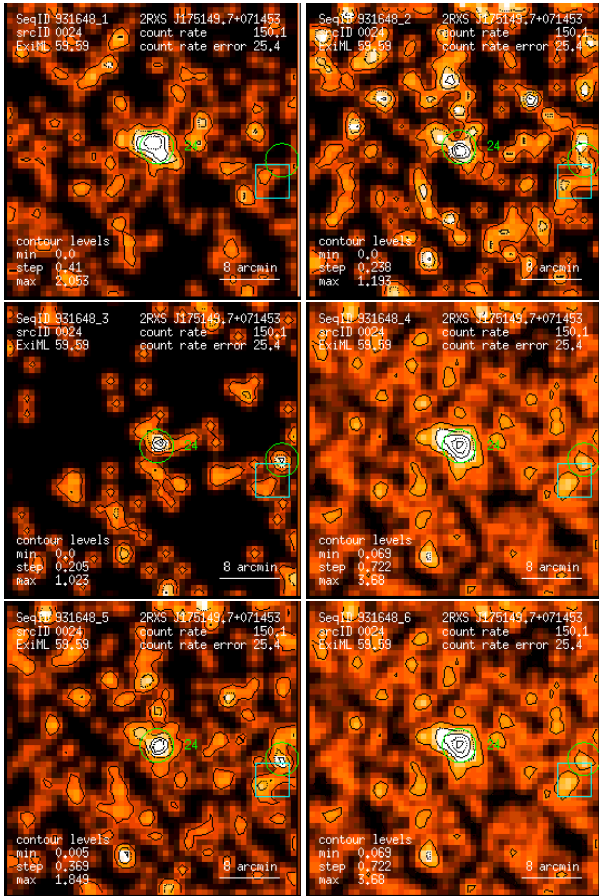
Figure 24: RASS 931648: detection 0024: band rate images, Gaussian filter: (1) PSPC channels 11 – 41, (2) 52 – 90, (3) 91 – 201, (4) 11 – 235, (5) 52 – 201, (6) 11 – 201. Broad band rates in counts/ks. Band rate contour levels in counts/ks/arcmin 2 .
