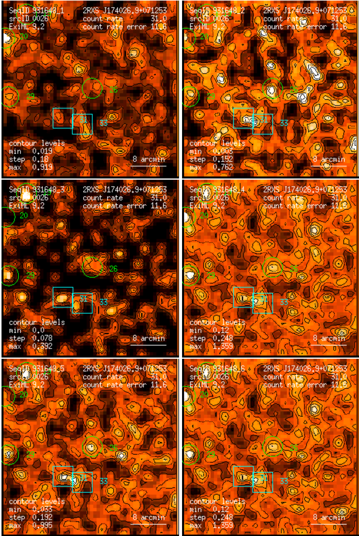
Figure 26: RASS 931648: detection 0026: band rate images, Gaussian filter: (1) PSPC channels 11 – 41, (2) 52 – 90, (3) 91 – 201, (4) 11 – 235, (5) 52 – 201, (6) 11 – 201. Broad band rates in counts/ks. Band rate contour levels in counts/ks/arcmin 2 .
