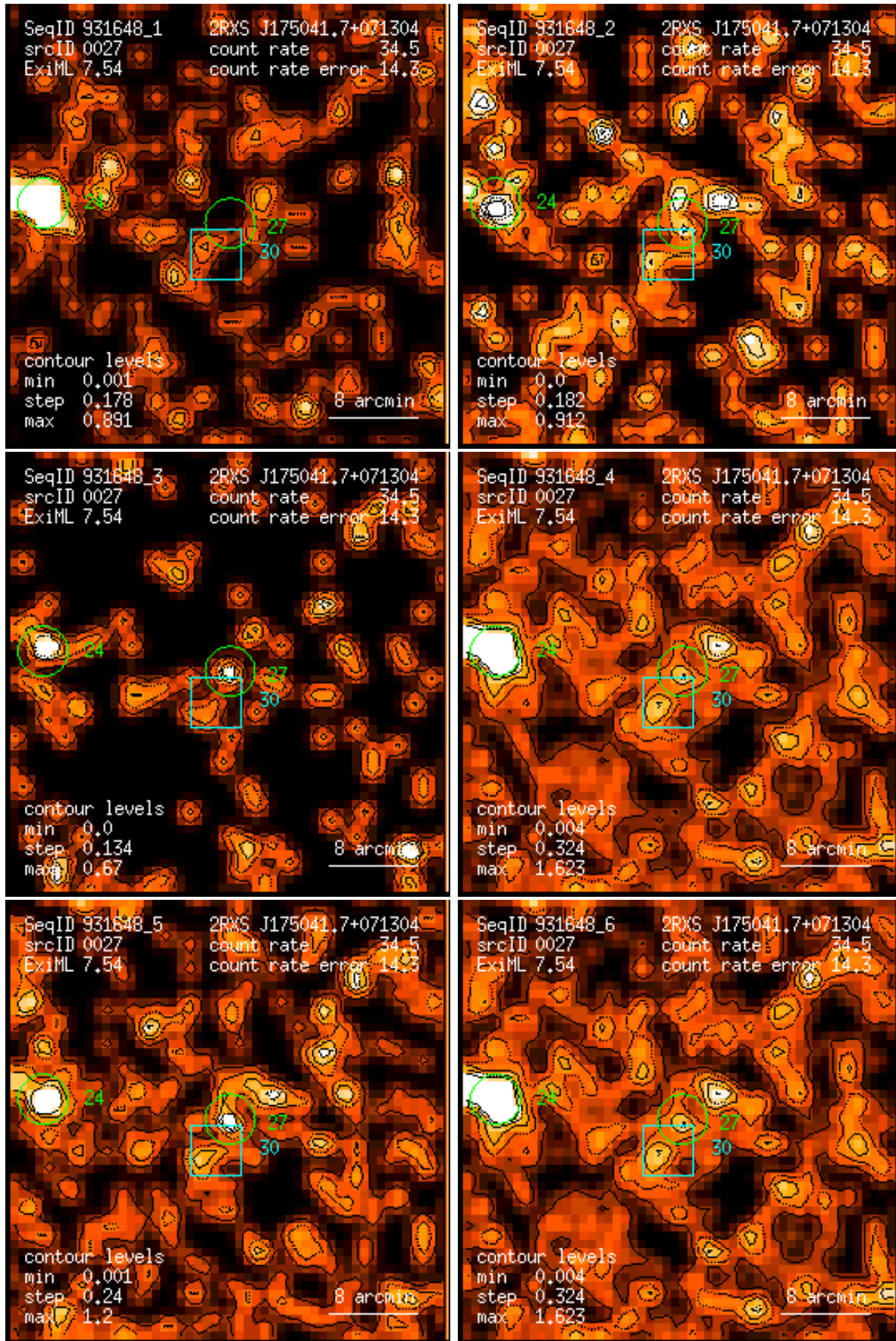
Figure 27: RASS 931648: detection 0027: band rate images, Gaussian filter: (1) PSPC channels 11 – 41, (2) 52 – 90, (3) 91 – 201, (4) 11 – 235, (5) 52 – 201, (6) 11 – 201. Broad band rates in counts/ks. Band rate contour levels in counts/ks/arcmin 2 .
