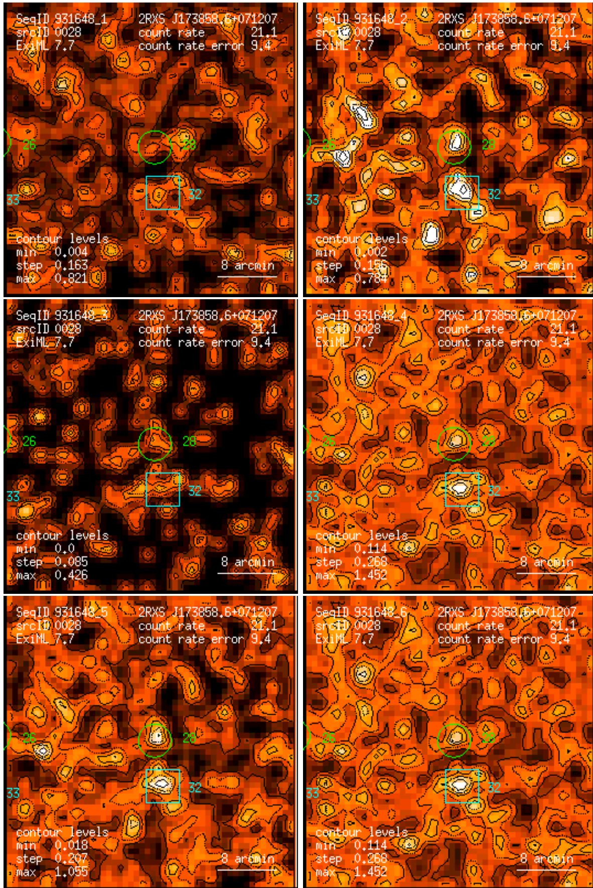
Figure 28: RASS 931648: detection 0028: band rate images, Gaussian filter: (1) PSPC channels 11 – 41, (2) 52 – 90, (3) 91 – 201, (4) 11 – 235, (5) 52 – 201, (6) 11 – 201. Broad band rates in counts/ks. Band rate contour levels in counts/ks/arcmin 2 .
