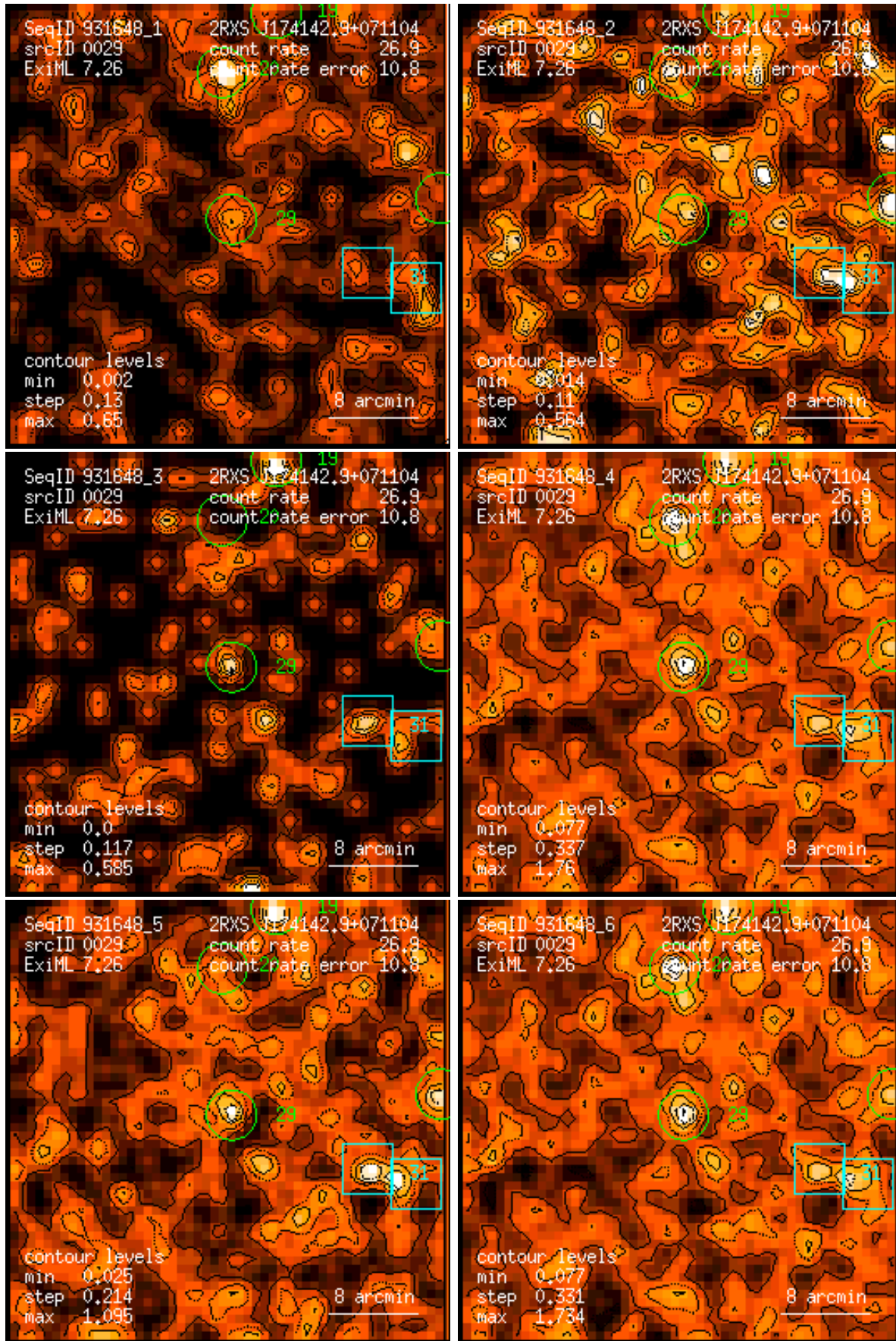
Figure 29: RASS 931648: detection 0029: band rate images, Gaussian filter: (1) PSPC channels 11 – 41, (2) 52 – 90, (3) 91 – 201, (4) 11 – 235, (5) 52 – 201, (6) 11 – 201. Broad band rates in counts/ks. Band rate contour levels in counts/ks/arcmin 2 .
