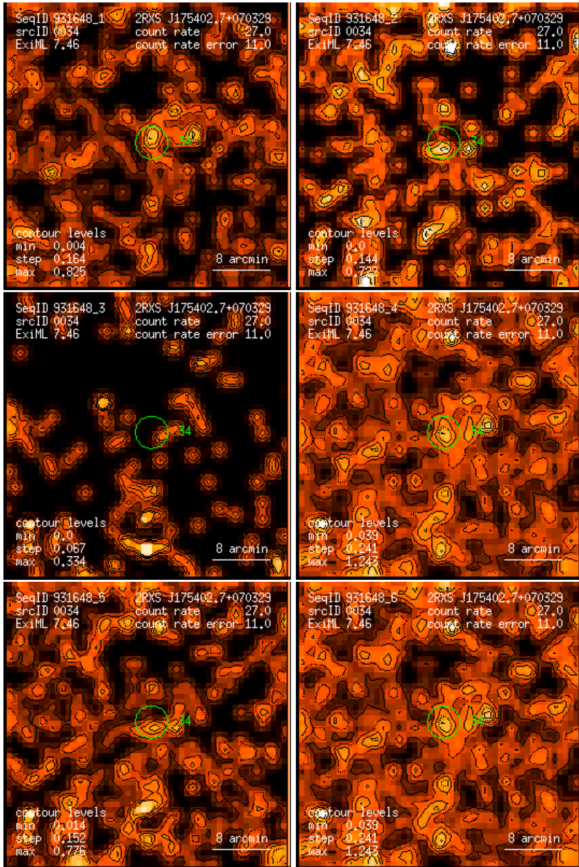
Figure 34: RASS 931648: detection 0034: band rate images, Gaussian filter: (1) PSPC channels 11 – 41, (2) 52 – 90, (3) 91 – 201, (4) 11 – 235, (5) 52 – 201, (6) 11 – 201. Broad band rates in counts/ks. Band rate contour levels in counts/ks/arcmin 2 .
