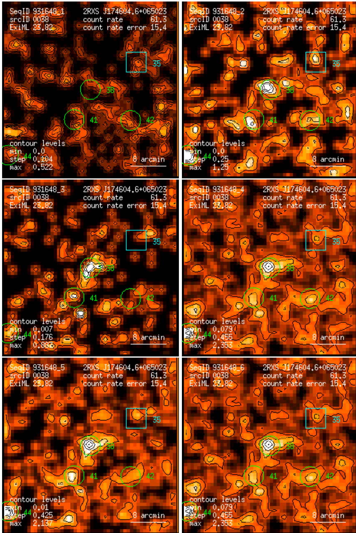
Figure 38: RASS 931648: detection 0038: band rate images, Gaussian filter: (1) PSPC channels 11 – 41, (2) 52 – 90, (3) 91 – 201, (4) 11 – 235, (5) 52 – 201, (6) 11 – 201. Broad band rates in counts/ks. Band rate contour levels in counts/ks/arcmin 2 .
