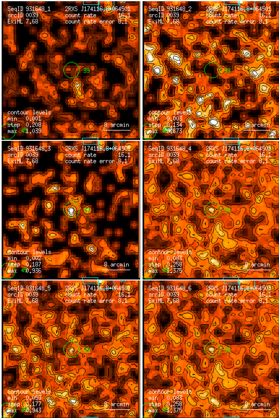
Figure 39: RASS 931648: detection 0039: band rate images, Gaussian filter: (1) PSPC channels 11 – 41, (2) 52 – 90, (3) 91 – 201, (4) 11 – 235, (5) 52 – 201, (6) 11 – 201. Broad band rates in counts/ks. Band rate contour levels in counts/ks/arcmin 2 .
