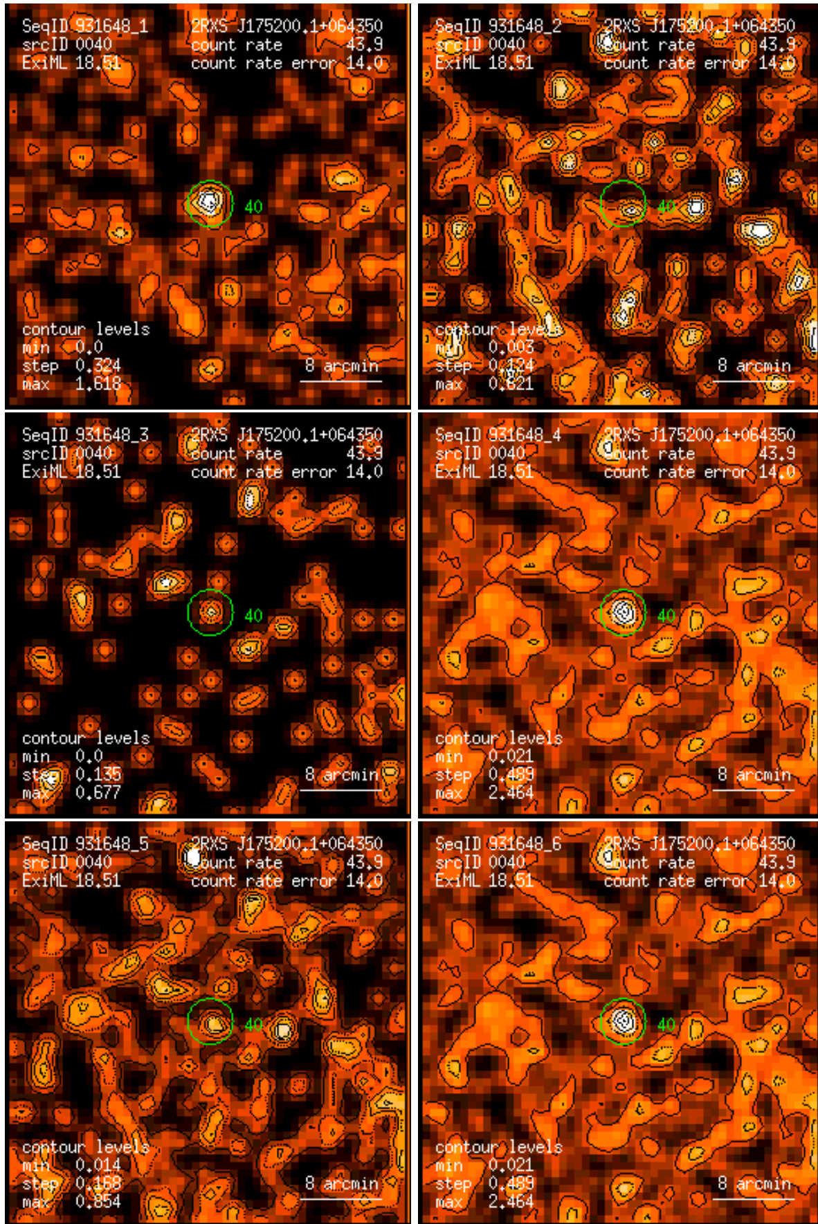
Figure 40: RASS 931648: detection 0040: band rate images, Gaussian filter: (1) PSPC channels 11 – 41, (2) 52 – 90, (3) 91 – 201, (4) 11 – 235, (5) 52 – 201, (6) 11 – 201. Broad band rates in counts/ks. Band rate contour levels in counts/ks/arcmin 2 .
