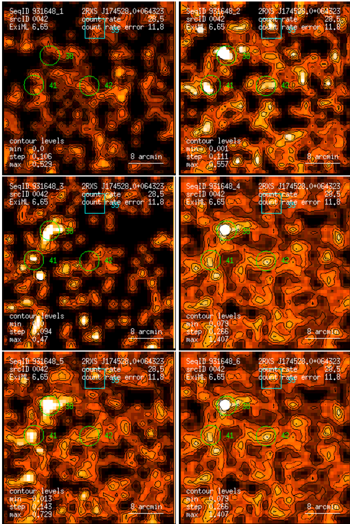
Figure 42: RASS 931648: detection 0042: band rate images, Gaussian filter: (1) PSPC channels 11 – 41, (2) 52 – 90, (3) 91 – 201, (4) 11 – 235, (5) 52 – 201, (6) 11 – 201. Broad band rates in counts/ks. Band rate contour levels in counts/ks/arcmin 2 .
