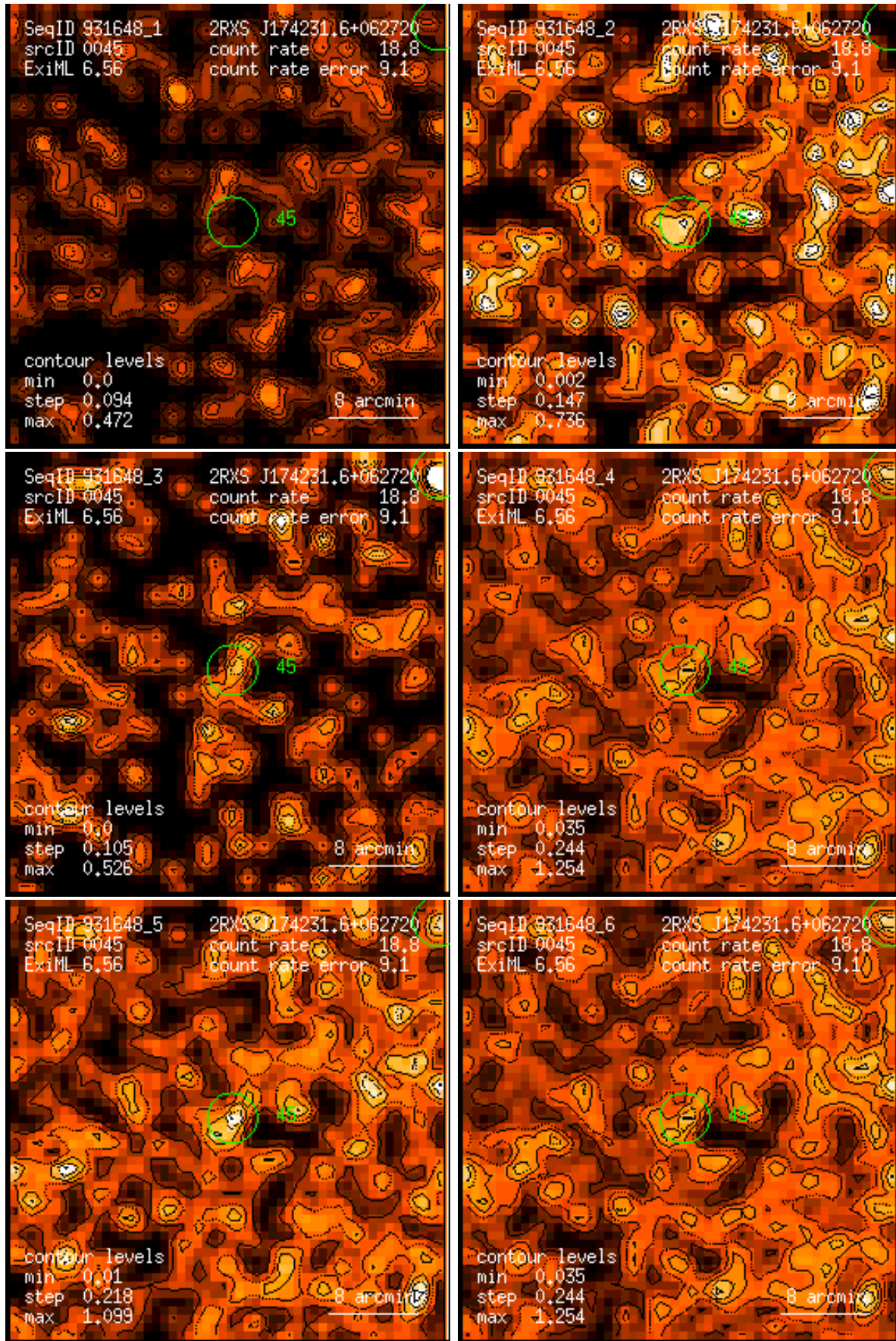
Figure 45: RASS 931648: detection 0045: band rate images, Gaussian filter: (1) PSPC channels 11 – 41, (2) 52 – 90, (3) 91 – 201, (4) 11 – 235, (5) 52 – 201, (6) 11 – 201. Broad band rates in counts/ks. Band rate contour levels in counts/ks/arcmin 2 .
