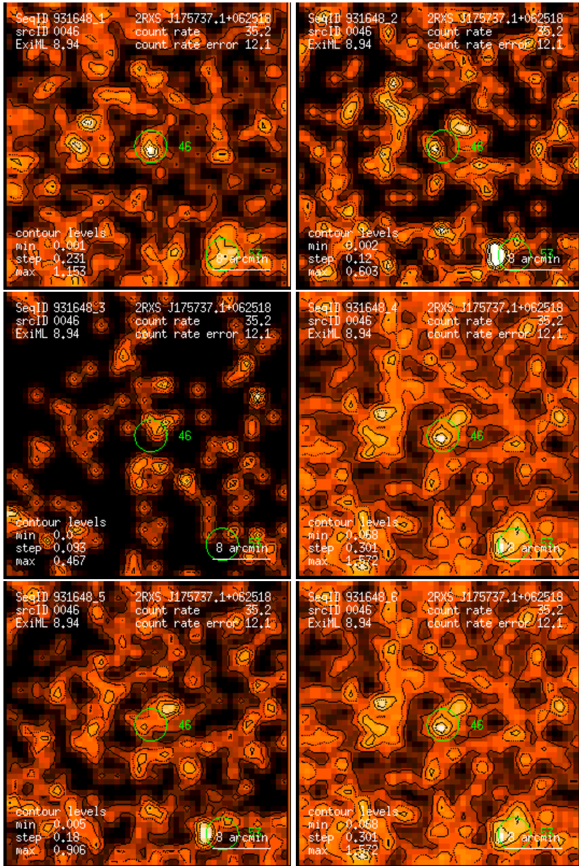
Figure 46: RASS 931648: detection 0046: band rate images, Gaussian filter: (1) PSPC channels 11 – 41, (2) 52 – 90, (3) 91 – 201, (4) 11 – 235, (5) 52 – 201, (6) 11 – 201. Broad band rates in counts/ks. Band rate contour levels in counts/ks/arcmin 2 .
