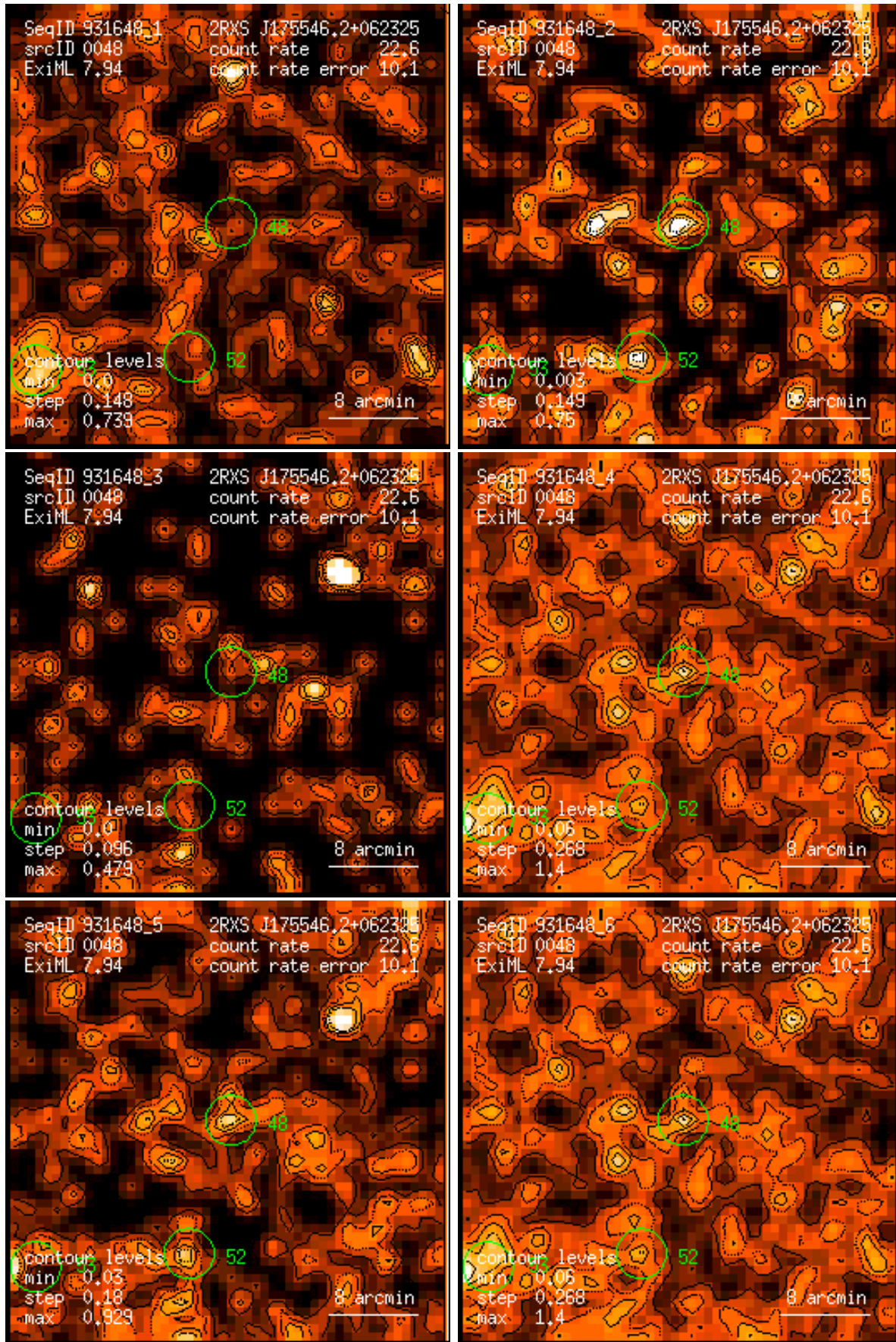
Figure 48: RASS 931648: detection 0048: band rate images, Gaussian filter: (1) PSPC channels 11 – 41, (2) 52 – 90, (3) 91 – 201, (4) 11 – 235, (5) 52 – 201, (6) 11 – 201. Broad band rates in counts/ks. Band rate contour levels in counts/ks/arcmin 2 .
